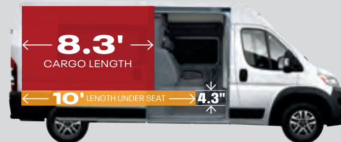
159-INCH WHEELBASE WITH CREW VAN PACKAGE
