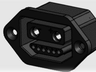
Female connector 2 power + 6 signal Battery pack
