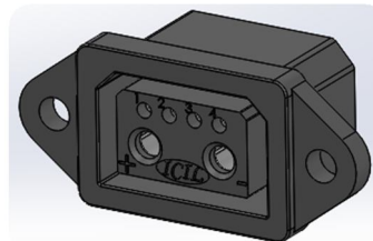
Female connector 2 power + 4 signal Battery pack
