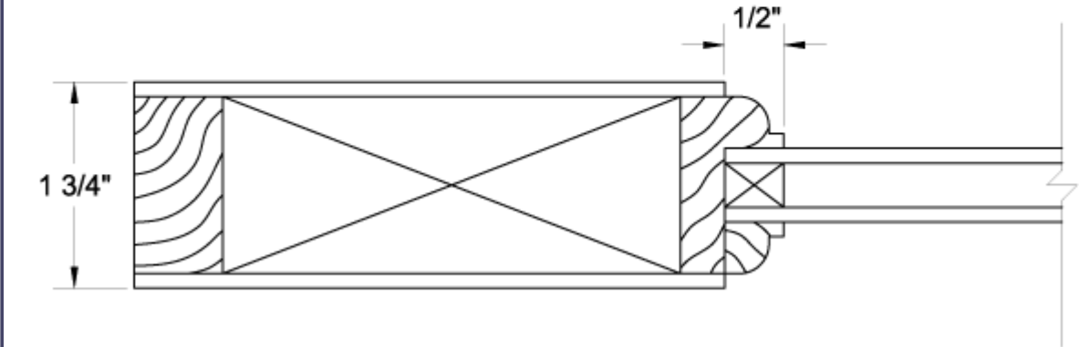
Ovolo Sticking (shown with 5/8" glass)
