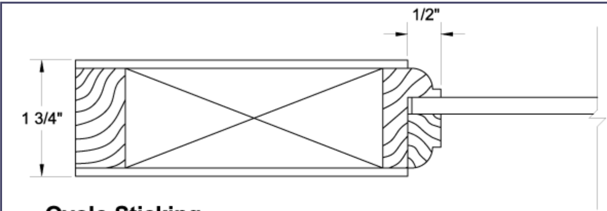
Ovolo Sticking (shown with 1/4" glass)
