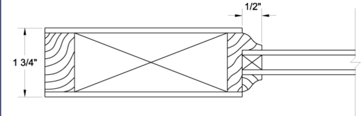
Ogee Sticking (shown with 5/8" glass)
