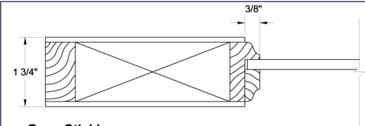
Ogee Sticking (shown with 1/4" glass)
