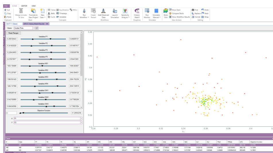
History match results (scatter plots)
