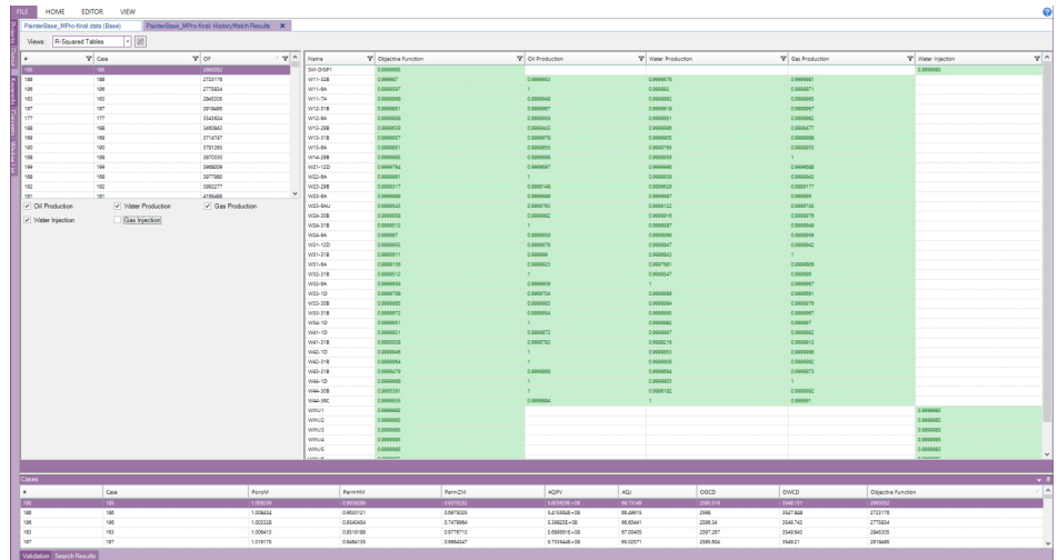
History match R-squared tables
