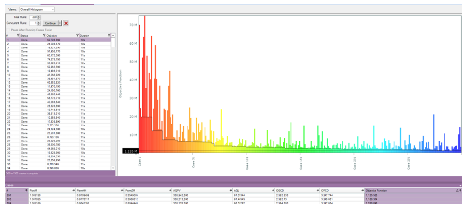
History match results (Overall histogram)
