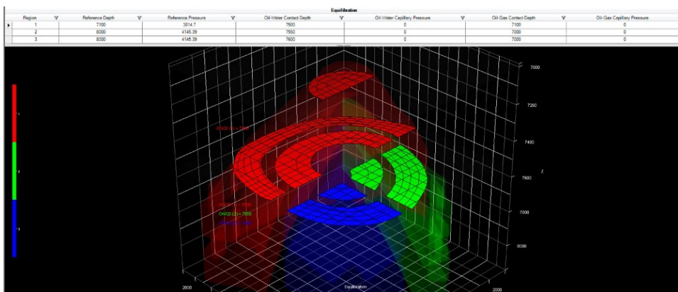
Equilibration view
