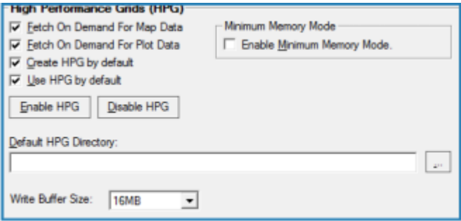
S3GRAF-HPG Options
