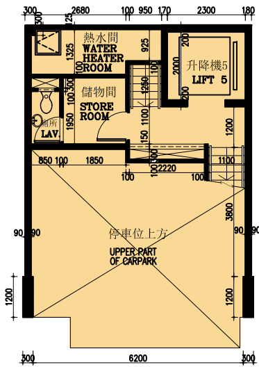
閣樓 MEZZ FLOOR
