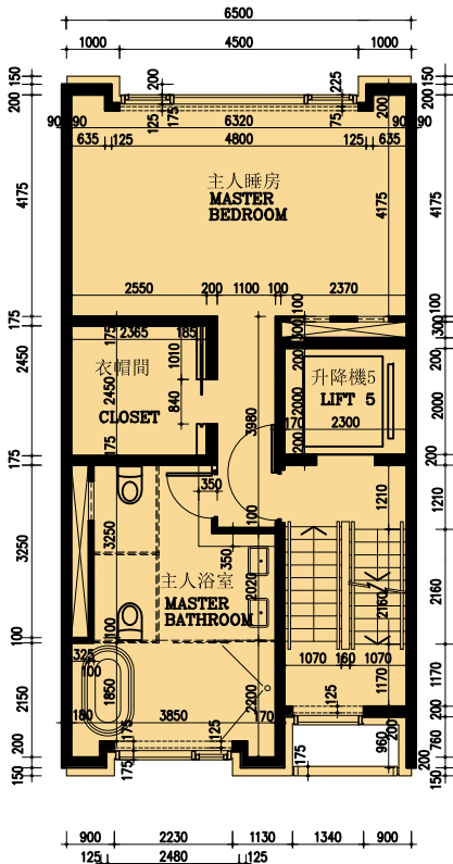
三樓 3RD FLOOR
