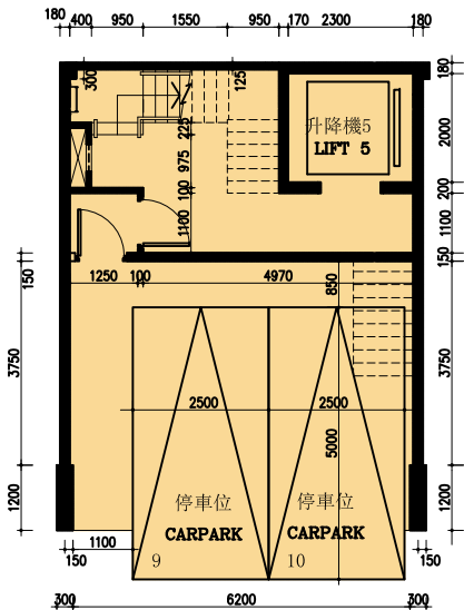
泊車層 CARPARK FLOOR
