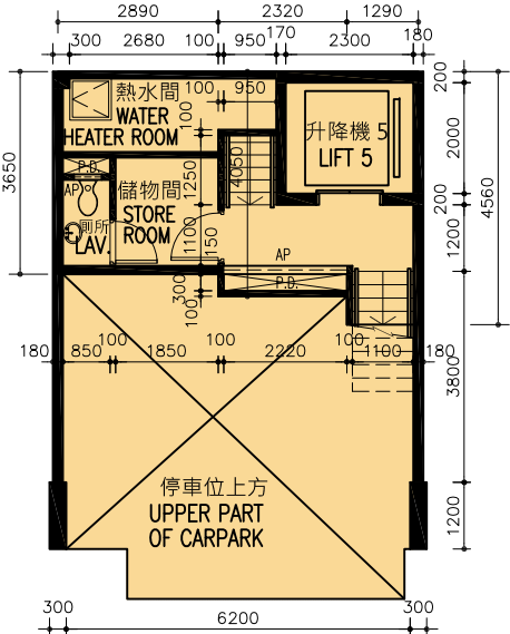
閣樓 MEZZANINE FLOOR
