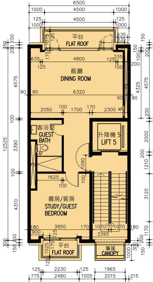
一樓 1ST FLOOR
