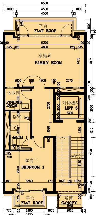
一樓 1ST FLOOR
