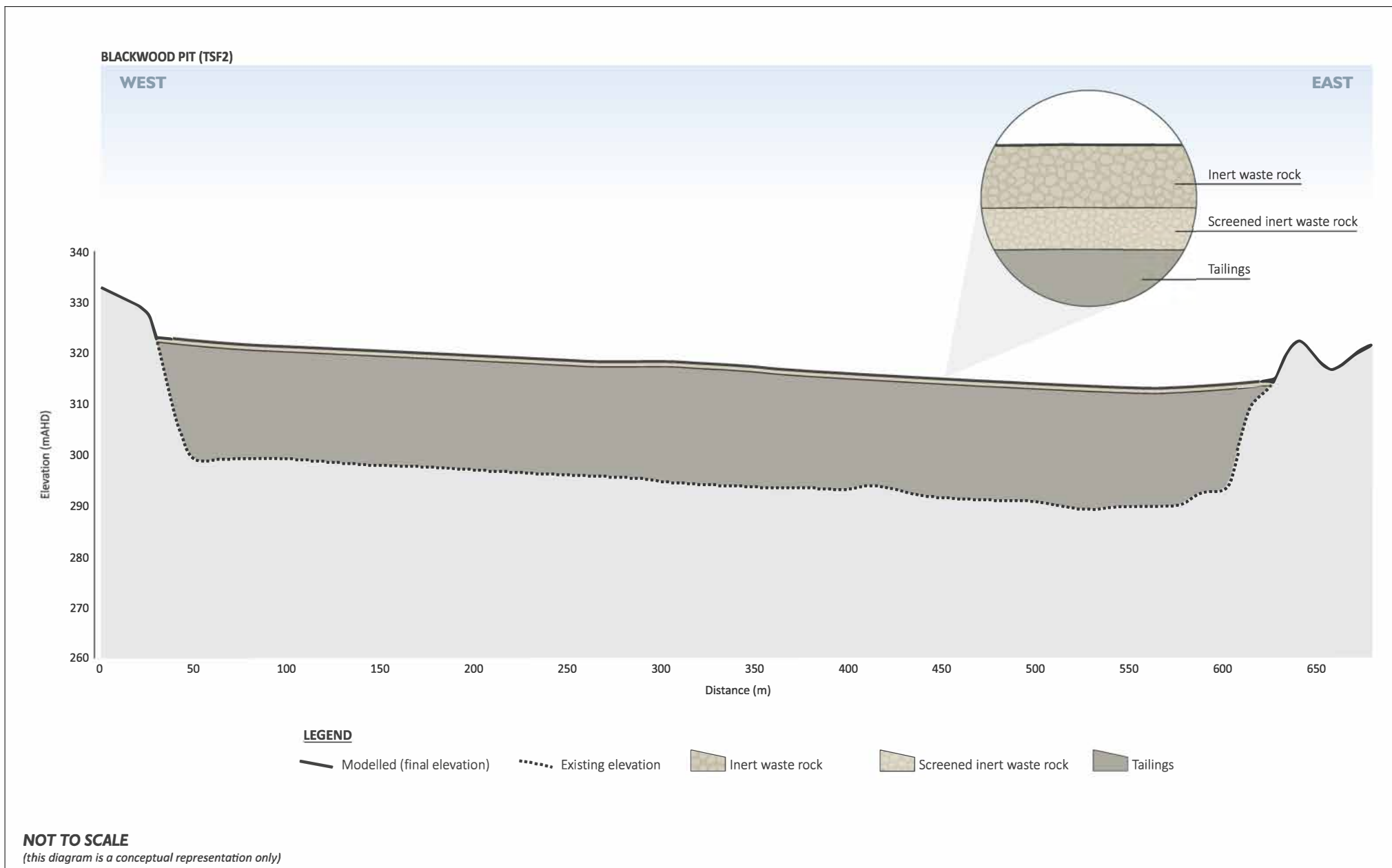
Blackwoods Pit (TSF2) final landform conceptual cross section
