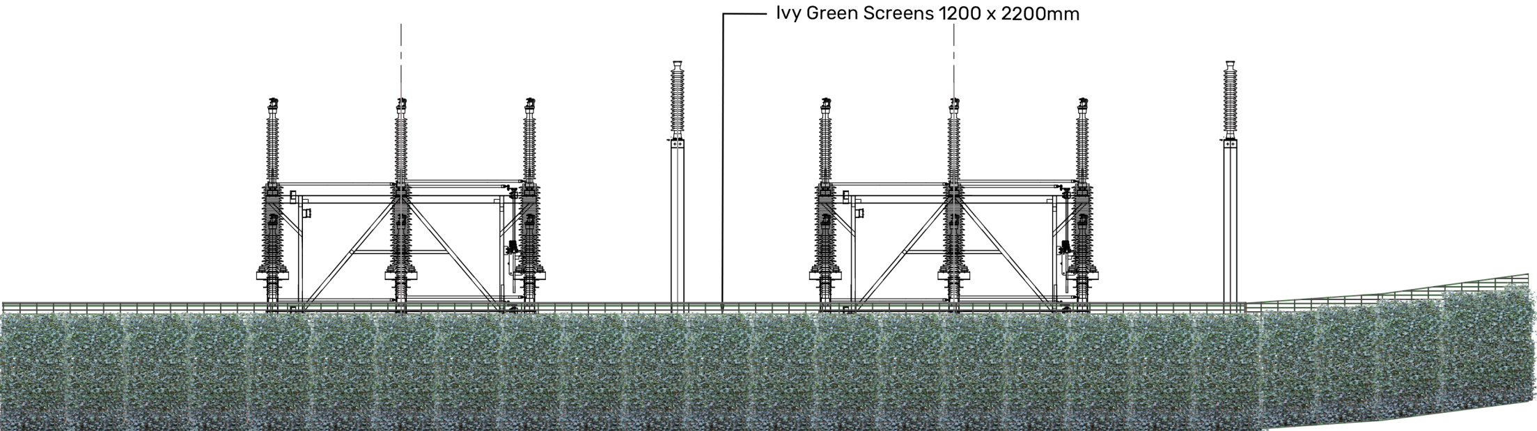
Section 2-2' 1:100
