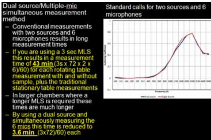
Figure 4.5. Comparison between single source and dual source/multiple-microphone measurement of the scattering coefficient. The agreement is excellent and the time reduction is quite dramatic.
