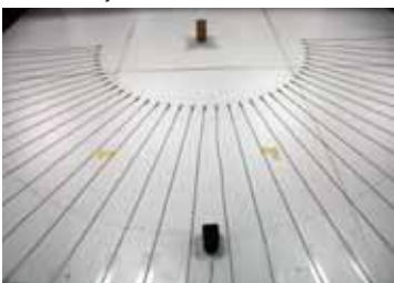
Figure 1.3 Diffusion Coefficient ISO 17497-2: How uniformly is the incident sound scattered (Can be measured in scale and calculated).
