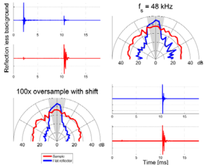
Figure 5.5. Top: Background subtraction without oversampling/shifting, shows residual direct sound in the reflection impulse response (blue) and resulting spikes in the reflector polar response. Bottom: Background subtraction with oversampling/shifting resulting in complete removal of the direct sound in the reflector and sample impulse responses, with accompanying smoothing of the reflector polar response.
