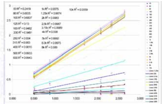
Figure 3.7. Correlation between area, perimeter and absorption. R. Sauro, M. Vargas, G. Mange, Internoise 2009 (Ottawa) Part 2.
