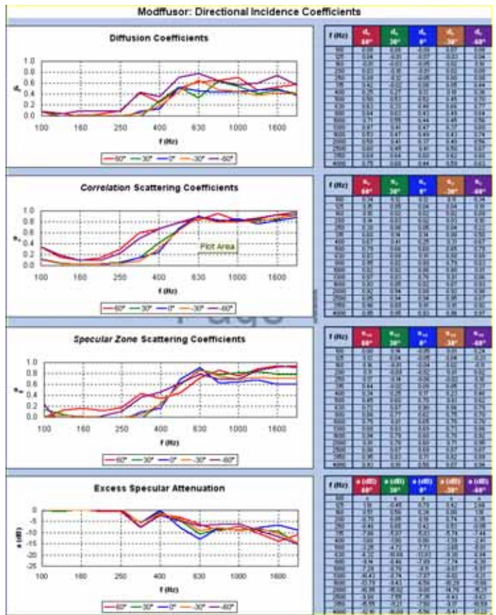
Figure 6.1. Directional Incidence Coefficients for the Moddfusor. responses are equal.
