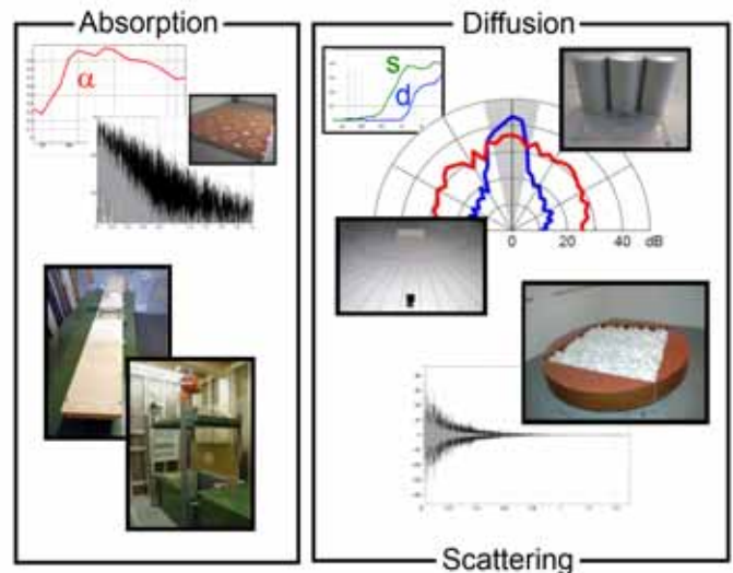
Figure 2.1 Measurement of the absorption coefficient, \alpha , is carried out using the rev room, top of Absorption panel, or normal incidence using the impedance tube method, shown in the lower area of the Absorption panel. Measurement of scattering surfaces is depicted in the right panel showing Diffusion and Scattering methodology. The scattering coefficient, s , can be obtained by the rotating table method shown in the lower area and by cross correlation of the sample and reflector polar responses shown in the upper area obtained using the goniometer method which also is used to determine the diffusion coefficient, d .
