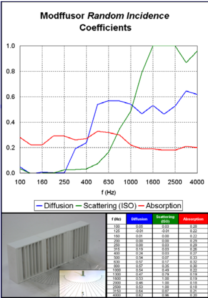
Figure 6.2. Random Incidence Coefficients for the Modffusor, along with tabulated data and a photo of the sample.
