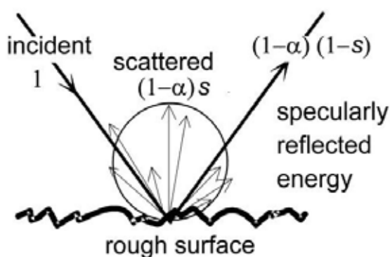
Figure 4.1. Graphic showing how incident sound, normalized to 1, can be specularly reflected and scattered. The scattering coefficient, s, determined the distribution.
