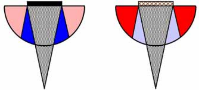
Figure 4.12. (left) Specular zone for a reflector in dark blue and the diffuse zone in light red; (right) Specular zone for a diffusor is shown in light blue and the diffuse zone in dark red, indicating energy is scattered out of the specular zone into the diffuse zone.
