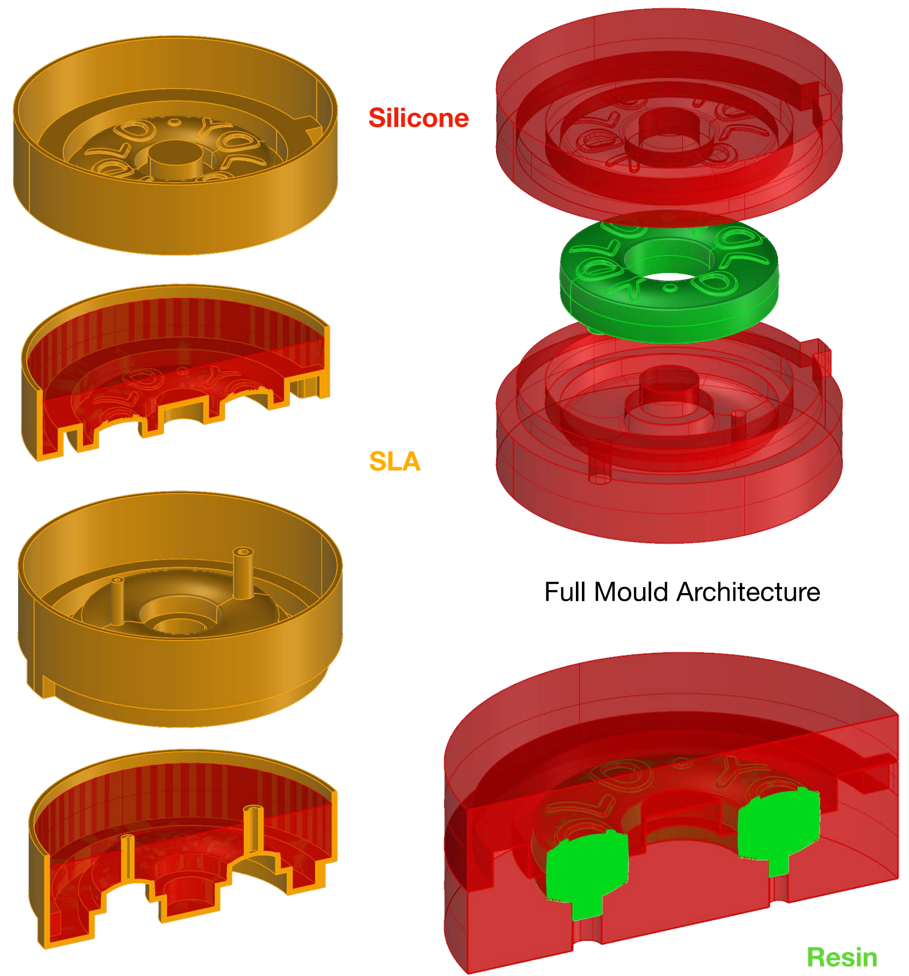
02 Part SLA reverse mould for silicone mould: This mould was used to produce multiple silicone moulds, helping speed up production by overcoming resin curing time limits. The reusable master mould allowed several silicone moulds to be made, which then enabled multiple resin parts to be cast simultaneously.
