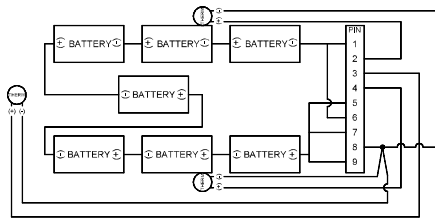
D717-01-100SMI Battery Pack Assembly
