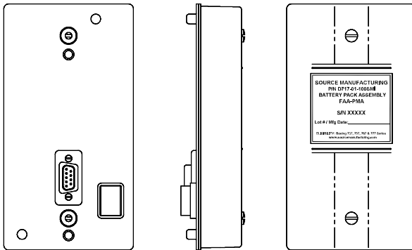
D717-01-100SMI Battery Pack Assembly
