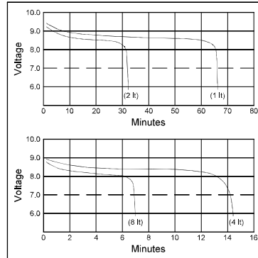
Typical Discharge Curves (7 Cell Pack)
