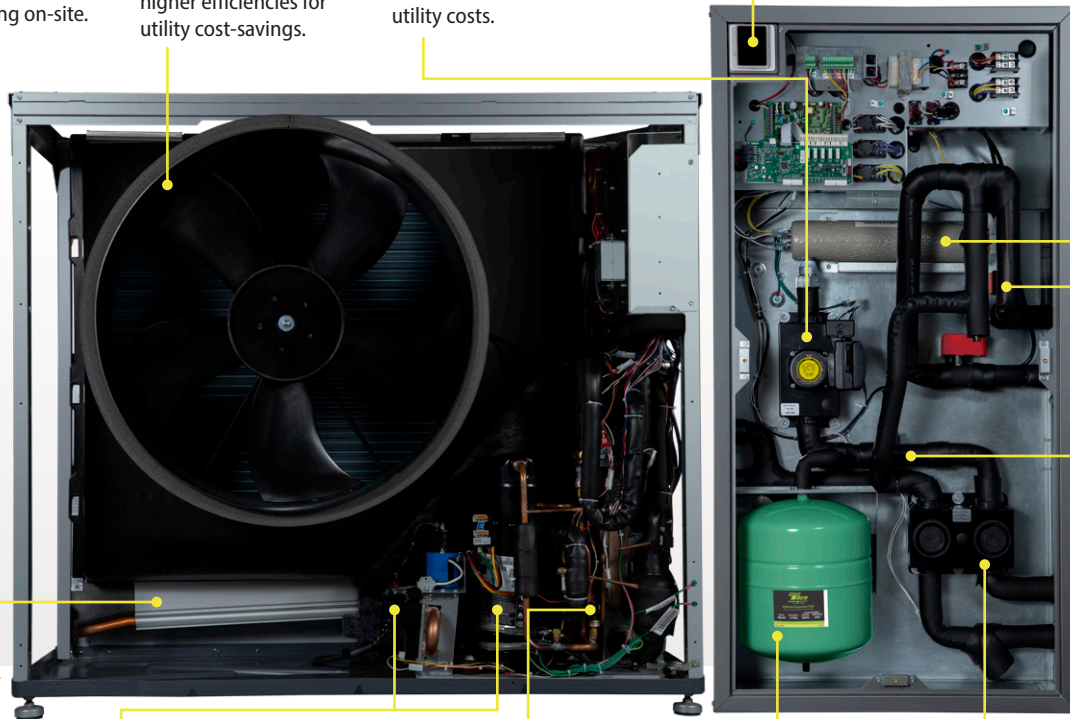
OUTDOOR UNIT
