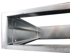
Above: Inside Standard Filter Housing. Rails for 1" or 2" filters.
