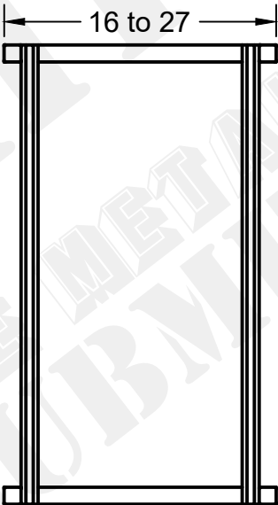
Top View
