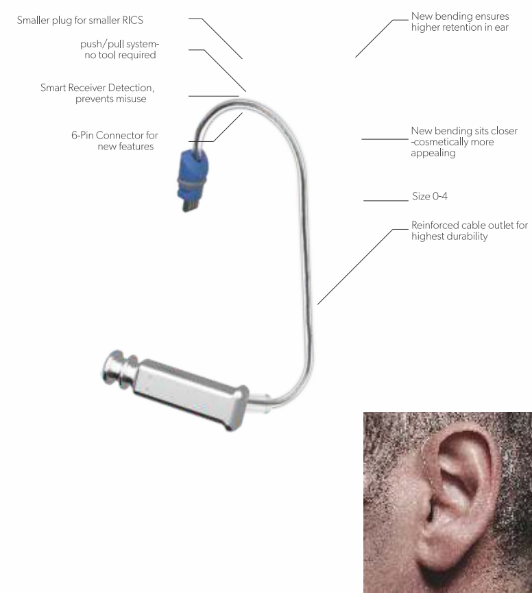
miniReceiver 3.0 Cable Bending 10/10 fit correctly-out of the box
