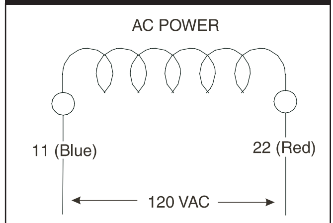
Figure 2.5 — Single Voltage, 1-Phase Stator Winding
