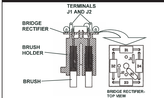
Figure 3.19 — Brush & Rectifier Combination
