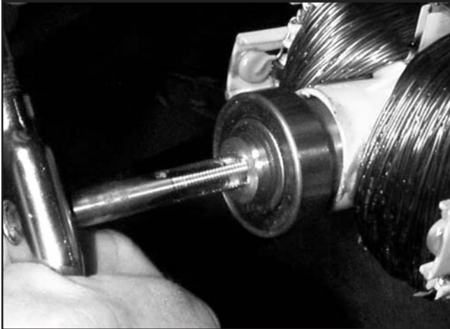
Figure 4.20 — Cutting Threads In The Rotor Shaft
