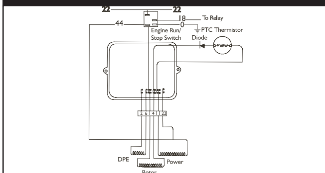
Figure 2.70 — Field Boost Assembly Schematic
