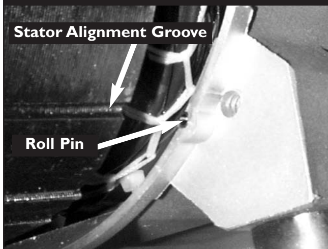
Figure 4.32 — Roll Pin To Stator Alignment
