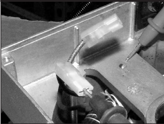
Figure 3.53 — Checking DPE “Short To Ground”
