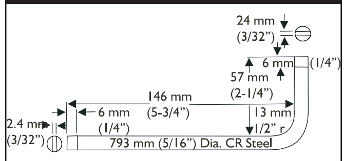
Figure 3.10 — Tang Bending Tool
