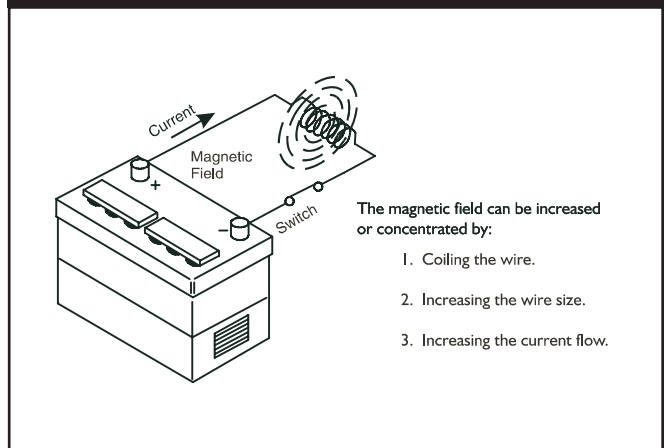
Figure 1.28 — Basic Principles Of Operation
