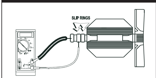
Figure 3.39 — Checking Rotor Short To Ground
