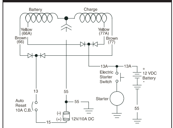
Figure 2.63 — Multi Tap Battery Charge Windings
