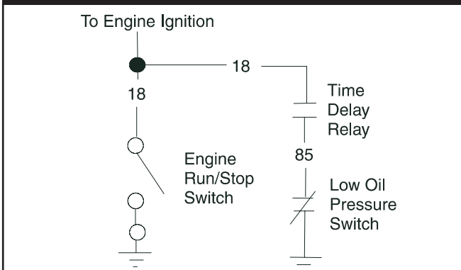
Figure 2.78 — V-Twin Time Delay Relay Schematic
