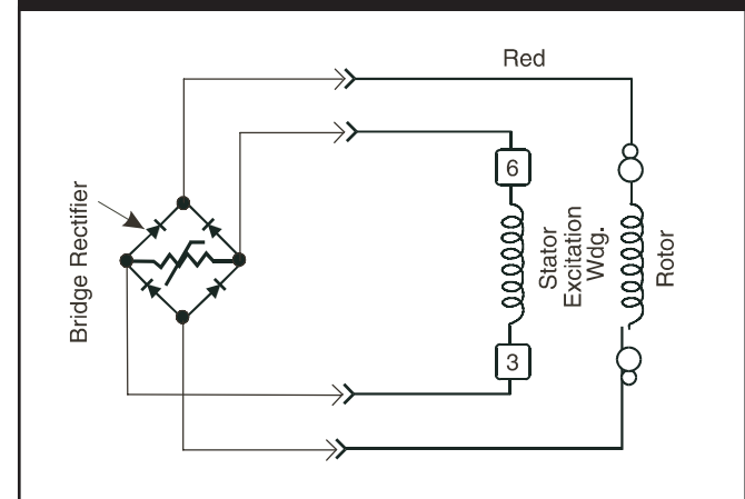
Figure 2.8 — Direct Excited Units
