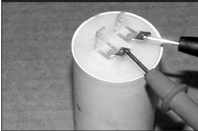
Figure 3.50 — Checking The Capacitor
