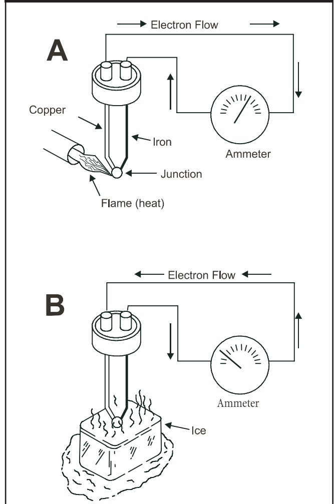
Figure 1.5 — The Thermocouple
