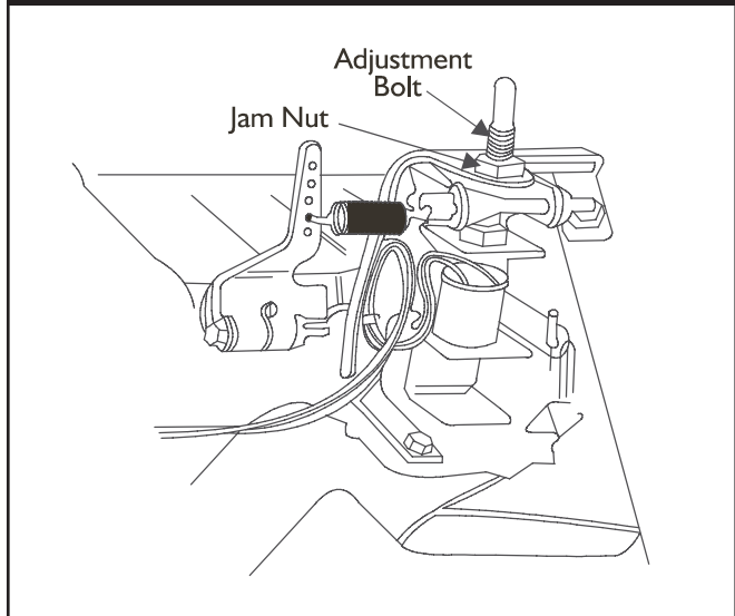
Figure 3.15 — Idle Control Solenoid
