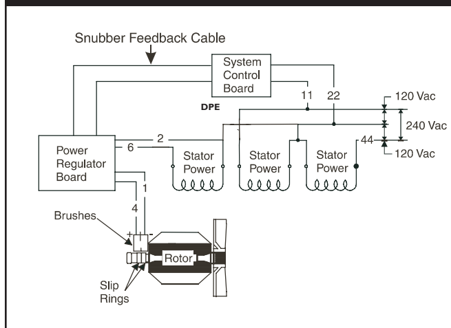
Figure 2.58 — Regulator And System Control Boards
