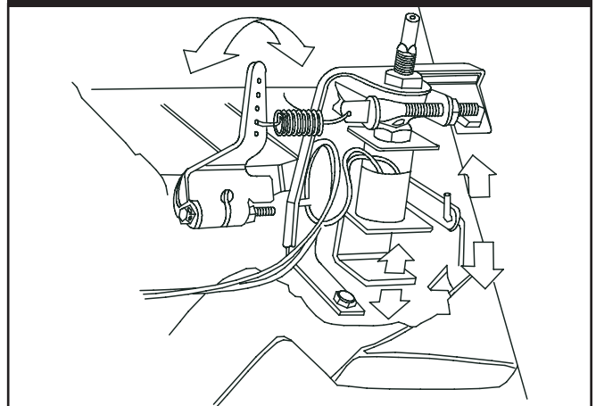
Figure 2.86 — GN-190 Governor And Idle Control
