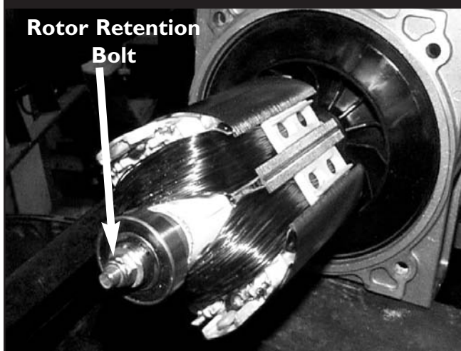
Figure 4.58 — Exposed Rotor Assembly
