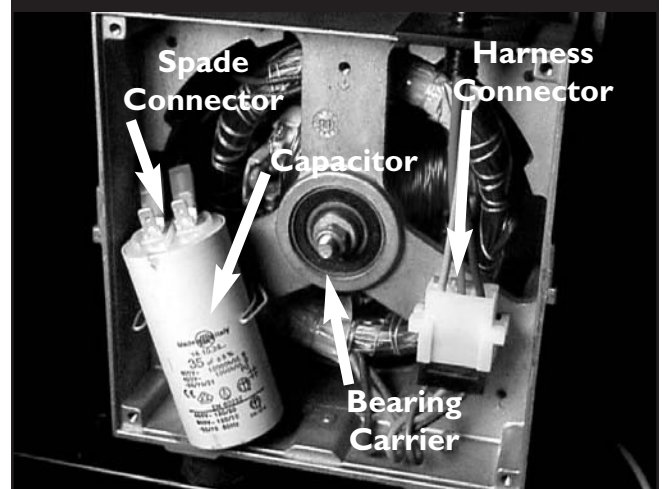
Figure 4.50 — Sincro® Components And Connections
