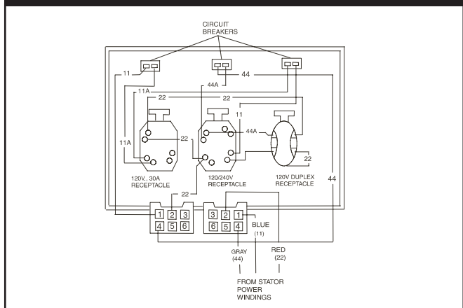
Figure 2.60 — Receptacles On Separate Control Panel
