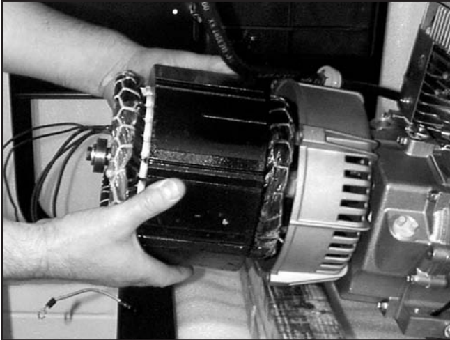
Figure 4.15 — Removing The Stator
