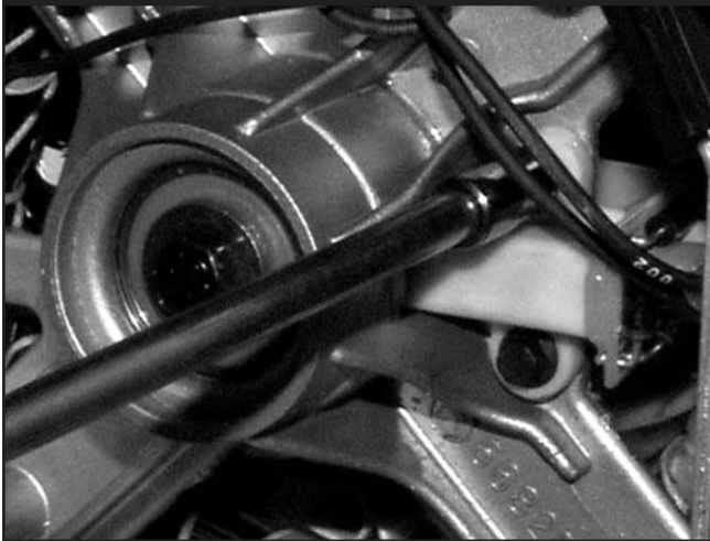
Figure 4.4 — Removing Brush Assembly
