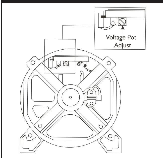
Figure 3.59 — Voltage Regulator
