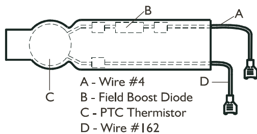
Figure 2.69 — Field Boost Assembly
