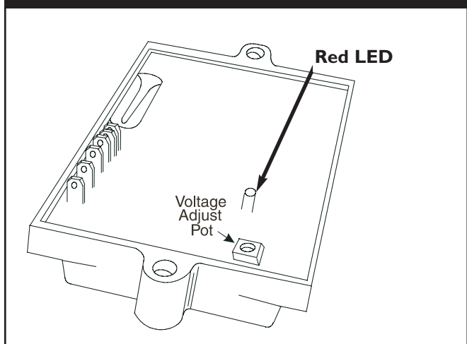
Figure 3.60 — Voltage Regulator
