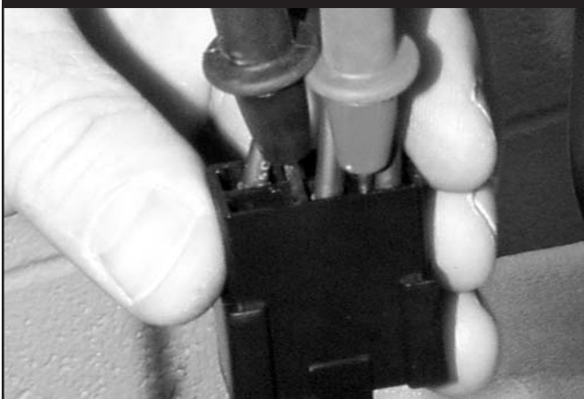
Figure 3.54 — Checking Power Winding Resistance
