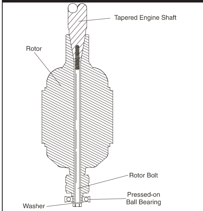
Figure 4.17 — Rotor Assembly... Cross Section
