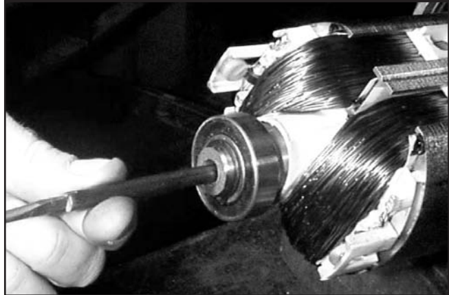
Figure 4.22 — Insert And Install Stud Into Tapered Shaft
