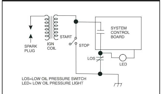
Figure 2.80 — "XL" Oil Pressure Switch Schematic
