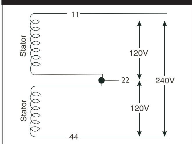
Figure 1.22 — Three Wire Circuit
