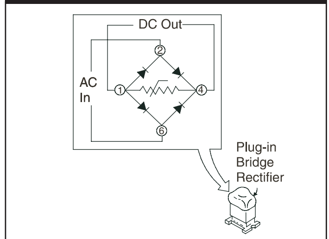
Figure 2.40 — Plug-In Bridge Rectifier With Varistor
