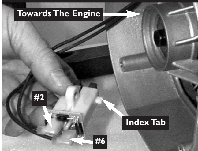
Figure 4.41 — Brush Assembly With Wire Terminals
