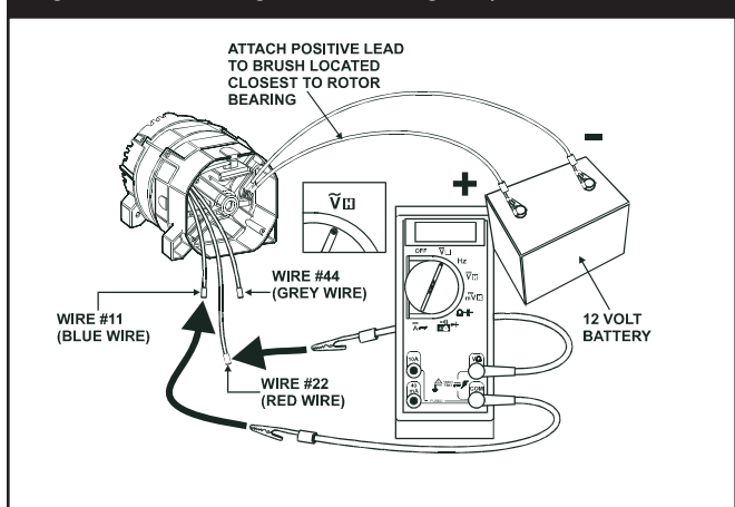
Figure 3.29 — Testing Power Winding Output
