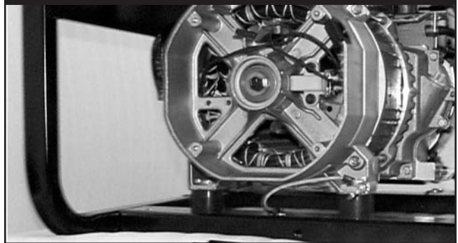
Figure 4.44 — Generator Vibration Mounts
