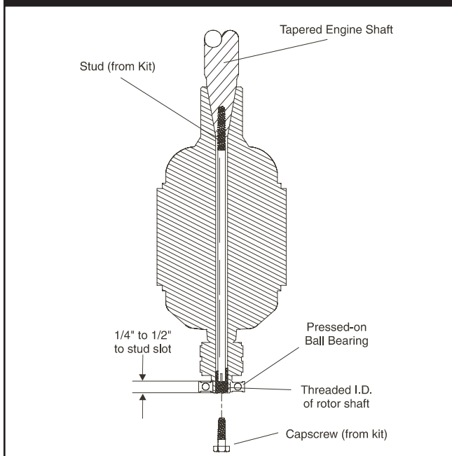
Figure 4.21 — Rotor Removal Kit Installation
