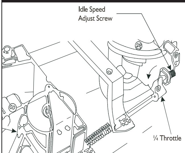
Figure 3.13 — Throttle Restrictor Tang
