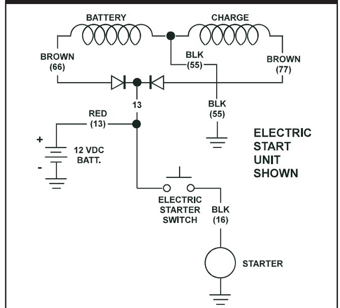
Figure 2.62 — Electric Start Unit
