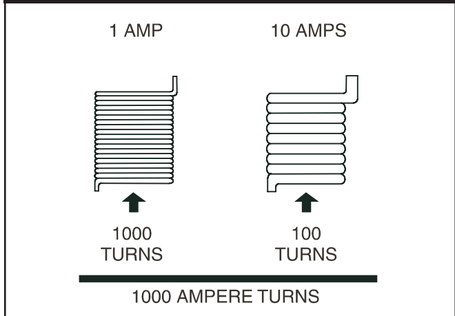
Figure I.13 — Example of “Ampere-Turns”
