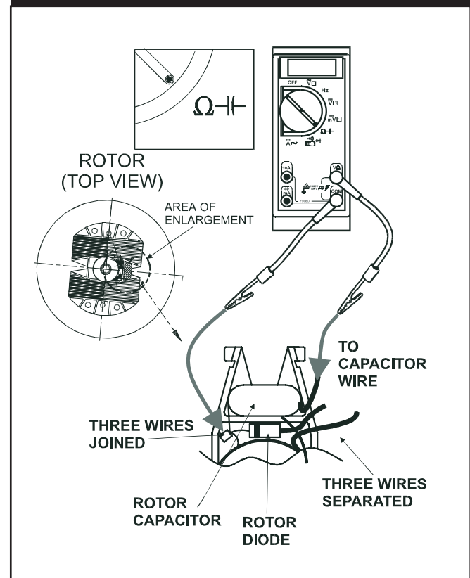
Figure 3.57 — Testing Rotor Capacitor
