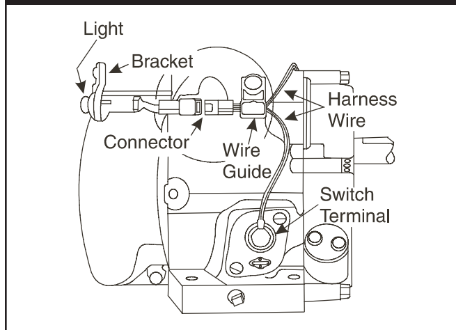
Figure 2.74 — Typical Low Oil Level System
