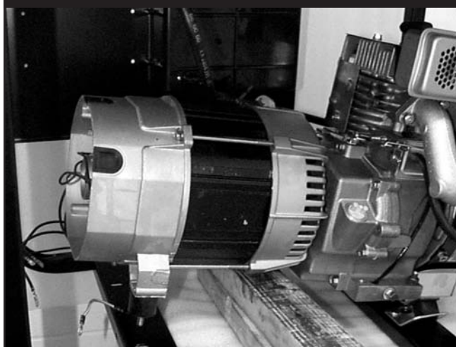
Figure 4.12 — Supporting The Generator
