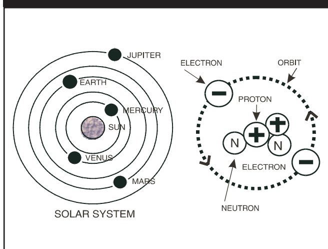
Figure I.1 — The Helium Atom
