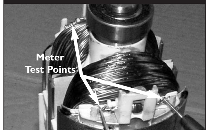
Figure 3.48 — Rotor Winding Resistance
