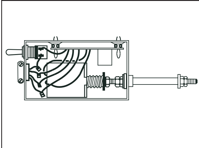
Figure 2.27 — Typical Idle Control Solenoid
