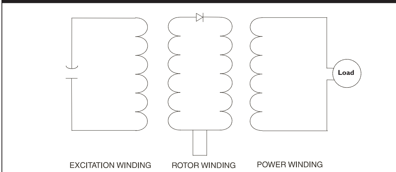
Figure 2.68 — A Brushless Excitation System
