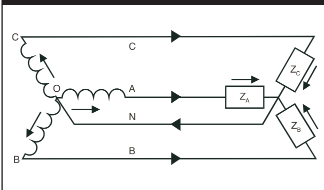
Figure I.24 — 4-Wire Wye Load (120 Volts Applied)
