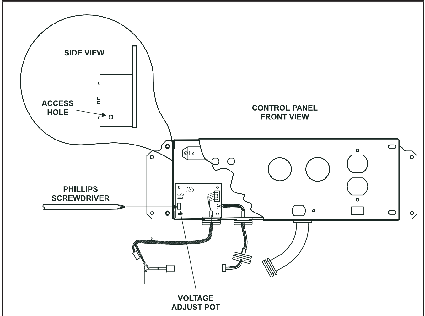
Figure 3.62 — Location Of The System Control Circuit & Access to The Voltage Control Pot
