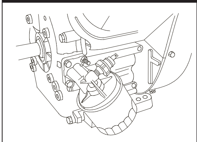
Figure 2.76 — The V-Twin Engine Pressure Switch
