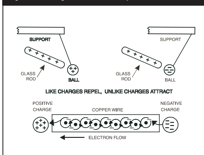
Figure I.2 — Magnetism and Electricity
