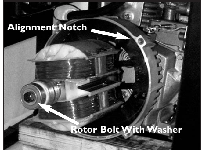
Figure 4.25 — Rotor In Housing
