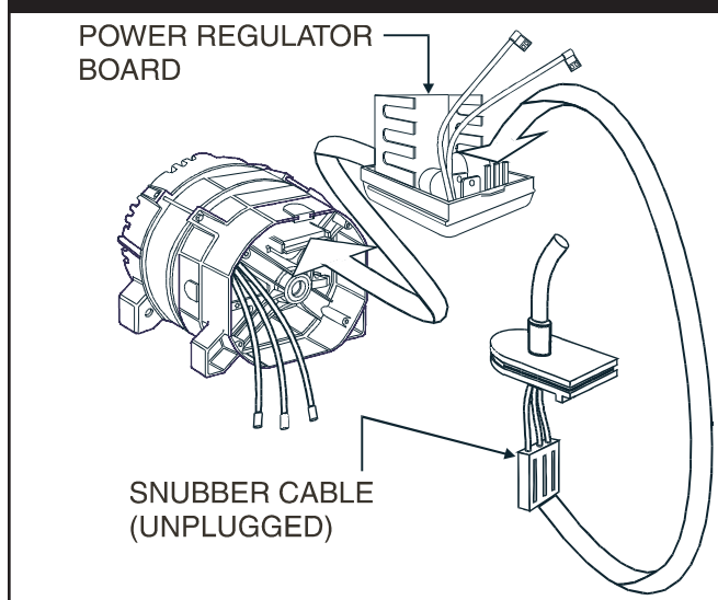
Figure 3.33 — Disconnecting Snubber Cable
