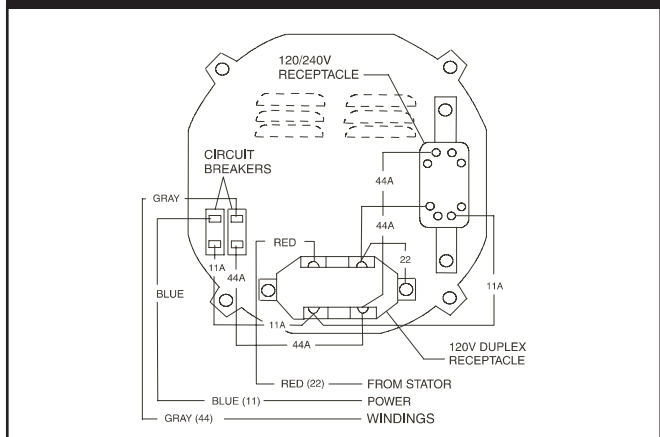
Figure 2.59 — Receptacles On Bearing Carrier Plate
