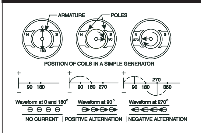
Figure I.14 — An Alternating Current Generator
