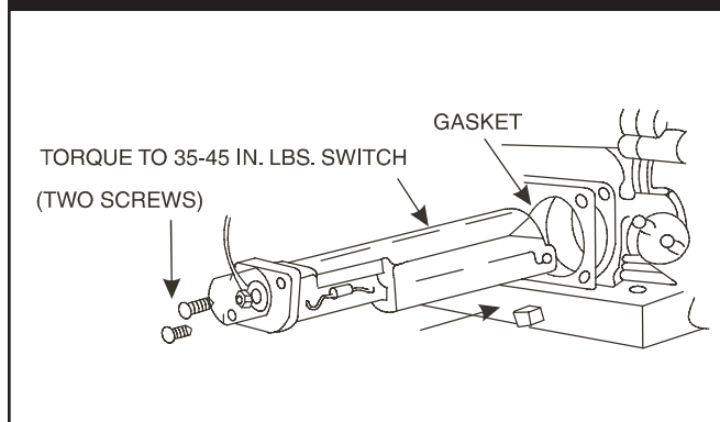
Figure 2.75 — Float Switch And Gasket
