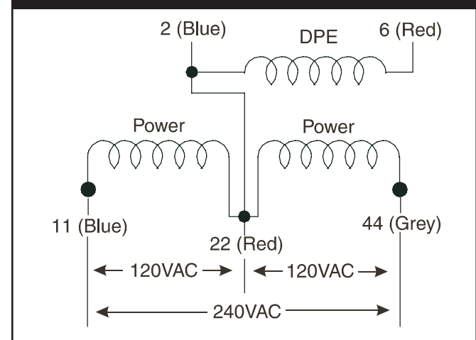
Figure 2.9 — (AC) / (DPE) Windings (“XL” and “MC”)
