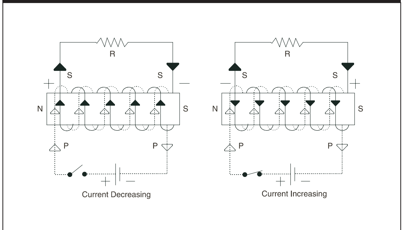
Figure 2.35 — The Principle Of Mutual Induction
