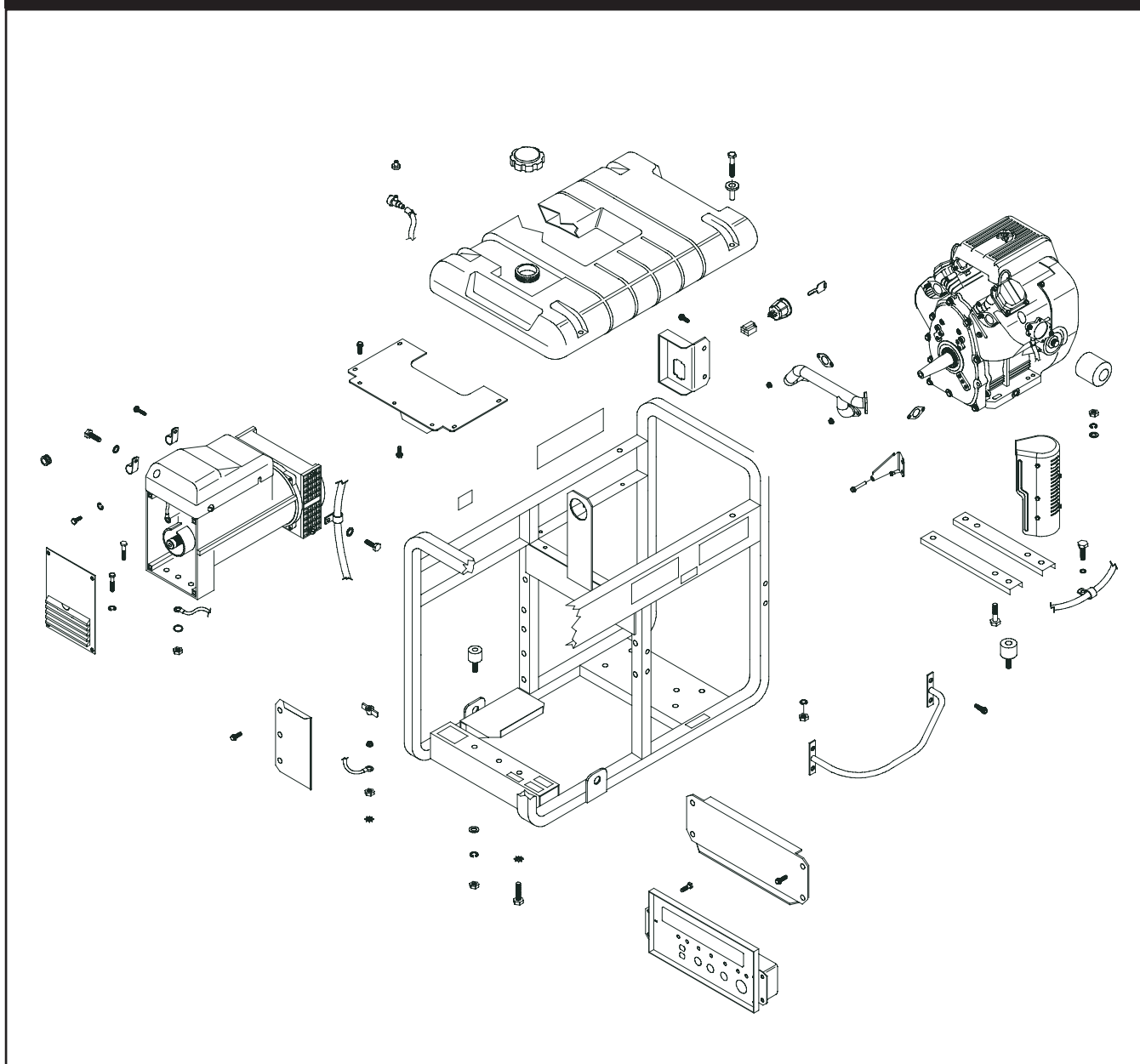
Figure 2.1 — Exploded View of a Typical Generator
