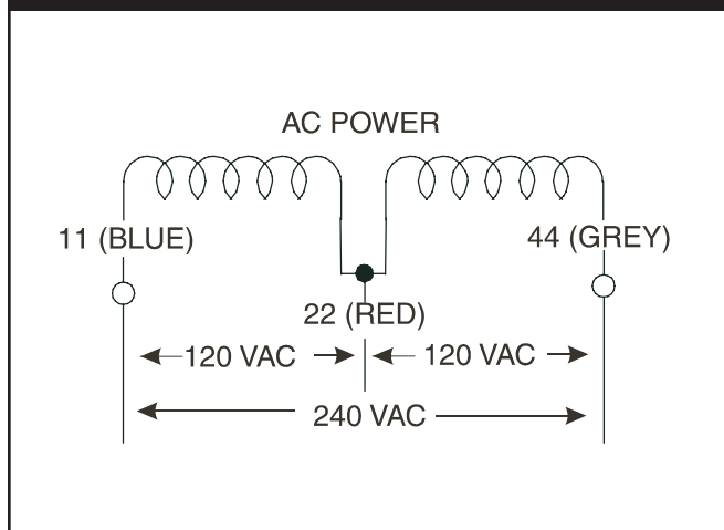
Figure 2.6 — Dual Voltage AC Power Winding
