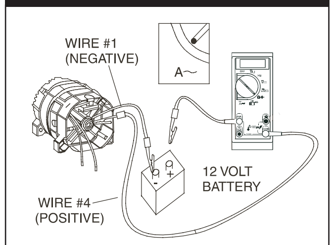
Figure 3.23 — Rotor Current Draw Test
