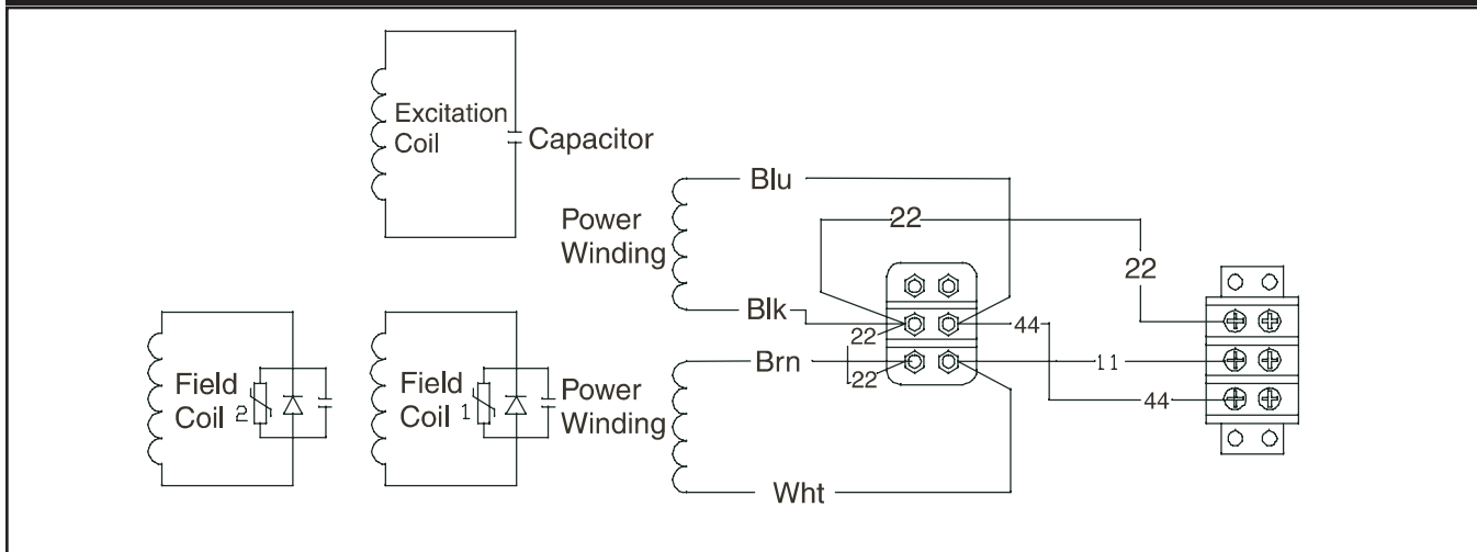
Figure 2.68 — A Brushless Excitation System
