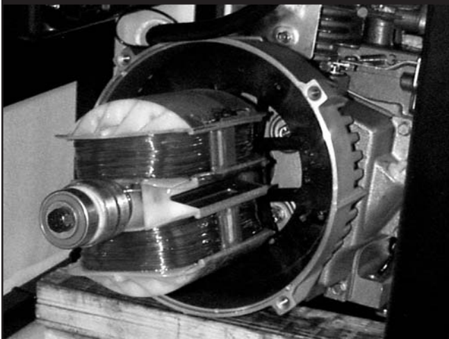
Figure 4.16 — Exposed Rotor
