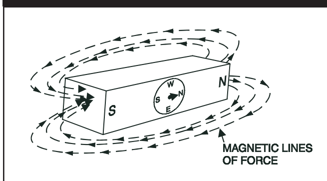
Figure I.6 — Lines of Flux Around A Magnet
