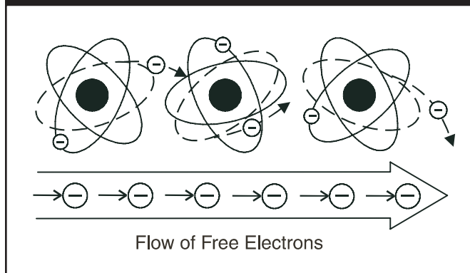
Figure I.3 — Transfer of Electrons
