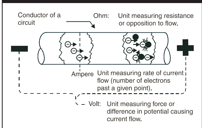
Figure I.16 — Electrical Measurement Units
