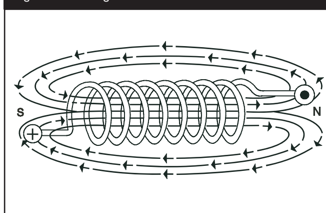
Figure 1.11 — Magnetic Field Around A Coil Of Wire
