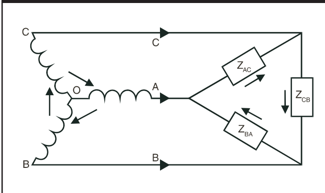
Figure I.25 — Load Connected In DELTA Fashion
