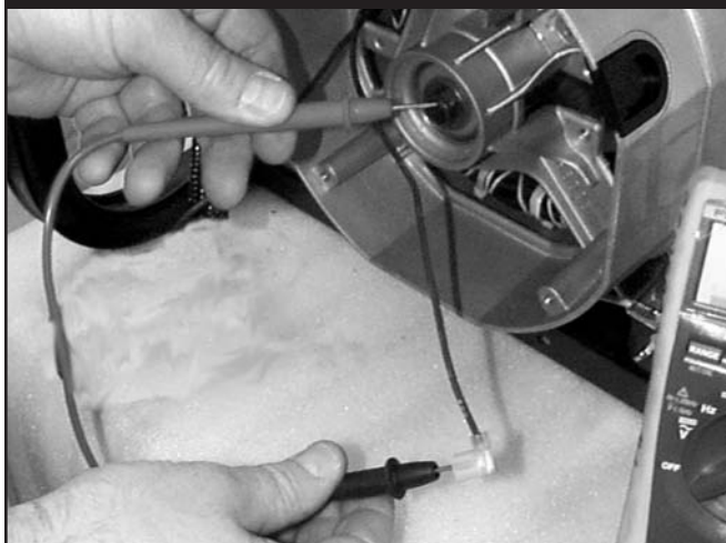
Figure 3.43 — Checking DPE “Short To Ground”
