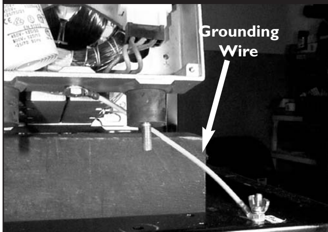
Figure 4.54 — Disconnect Frame Grounding Wire
