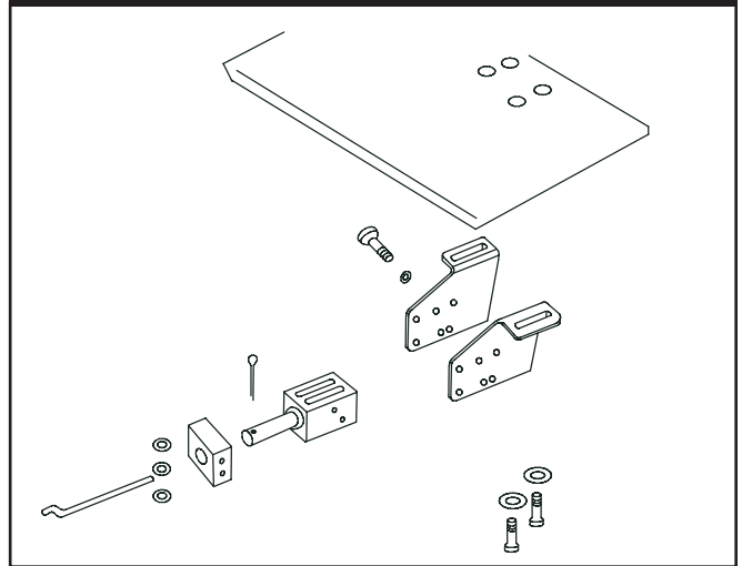
Figure 2.85 — V-Twin Idle Control Solenoid
