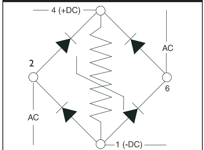
Figure 2.46 — Bridge Rectifier Schematic
