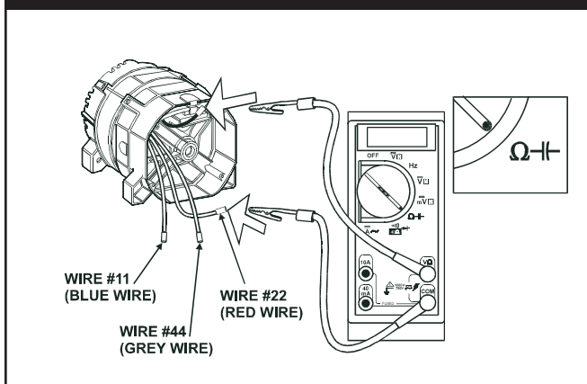
Figure 3.42 — Testing For Continuity Between Windings
