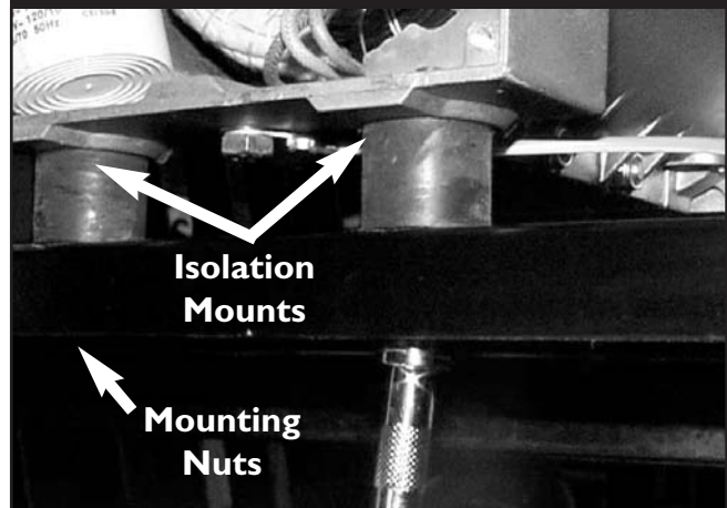
Figure 4.52 — Isolation Mount Hardware
