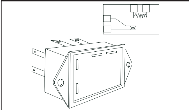
Figure 2.77 — V-Twin Engine's Time Delay Relay
