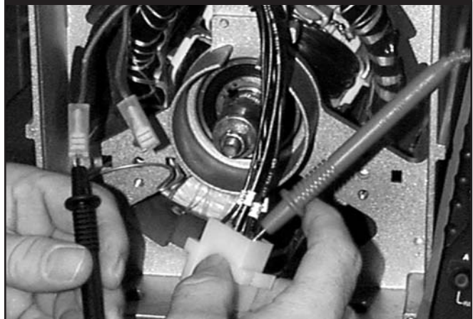
Figure 3.52 — Testing For Short Between Windings
