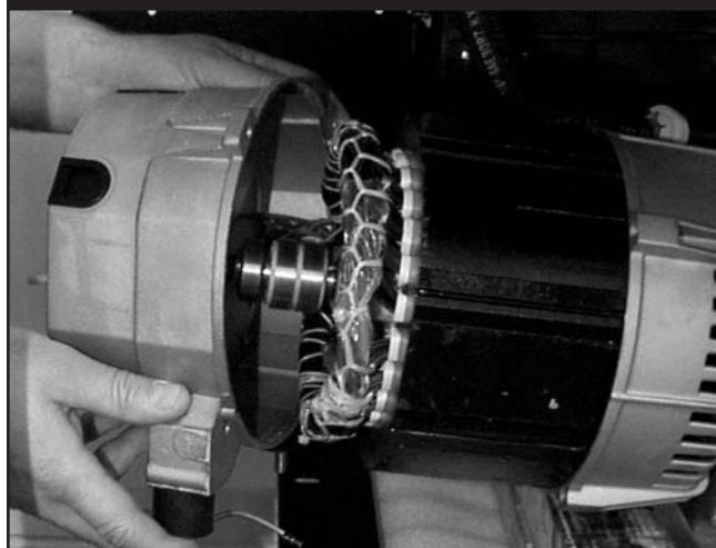
Figure 4.14 — Removing Rear Bearing Carrier
