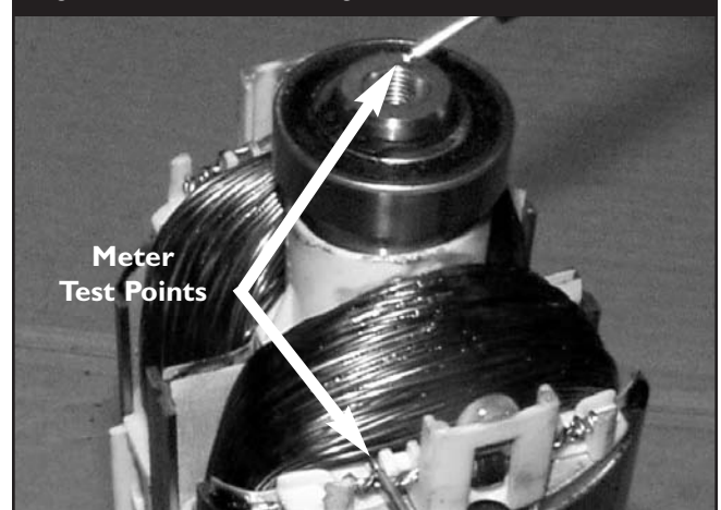
Figure 3.49 — Rotor Winding Resistance
