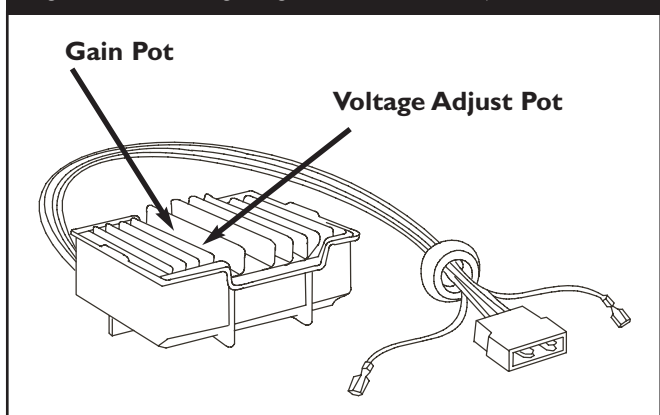
Figure 3.61 — Voltage Regulator With Gain Adjust
