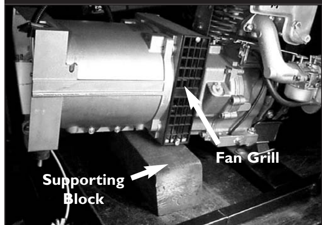
Figure 4.53 — Supporting Sincro-Generator
