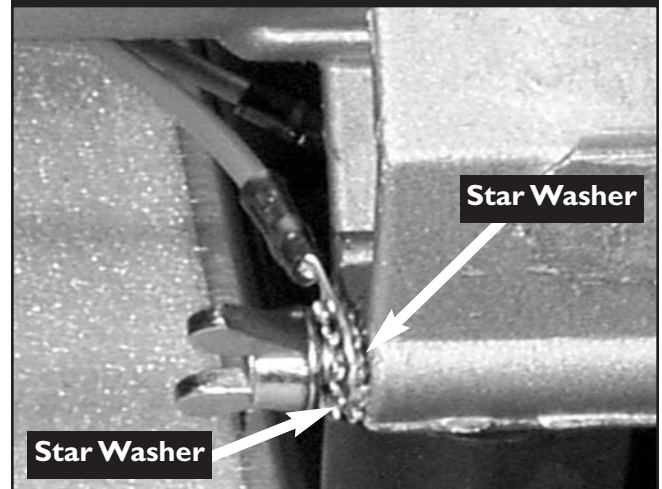
Figure 4.40 — Grounding Connection
