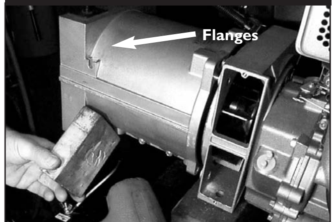
Figure 4.57 — Tapping Stator Housing Flanges
