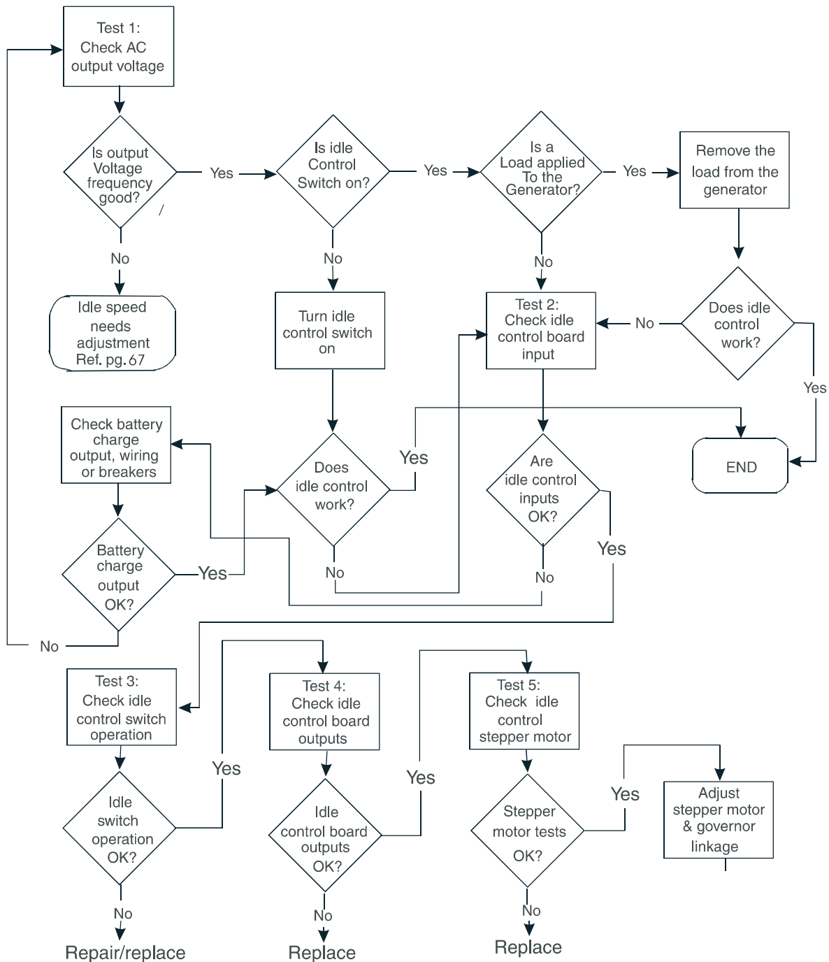
Figure 3.4 — Idle Control Troubleshooting Flow Chart (480 & 570 V-Twin GN Engines 8000-10000 Watt Generators)
