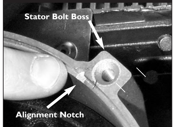
Figure 4.26 — Engine Adapter Housing Alignment
