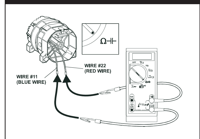
Figure 3.44 — Checking Power Winding Resistance
