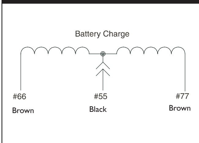
Figure 2.10 — Stator Battery Charge Circuit
