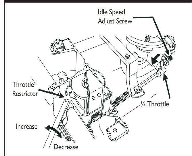
Figure 3.12 — Throttle Restrictor Tang
