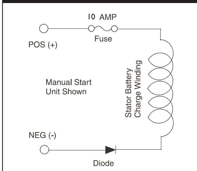
Figure 2.61 — Battery Charge Windings (BCW)
