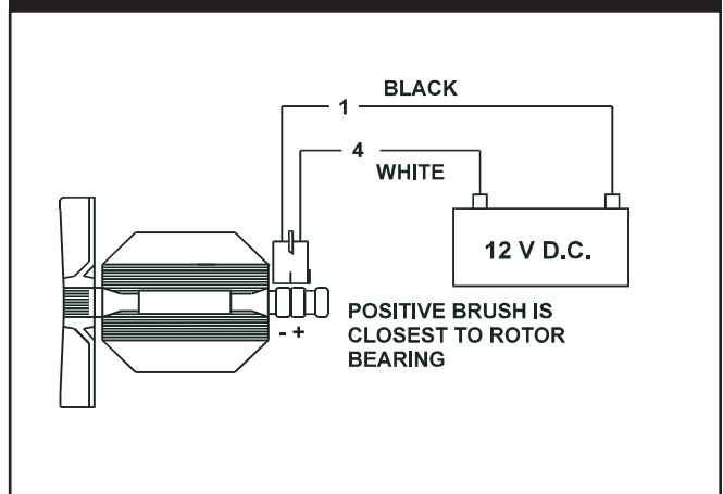
Figure 3.32 — Restoring Residual Magnetism
