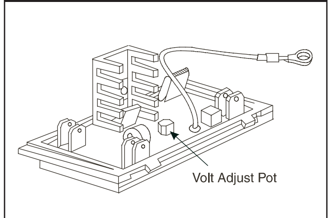
Figure 2.52 — Voltage Regulator
