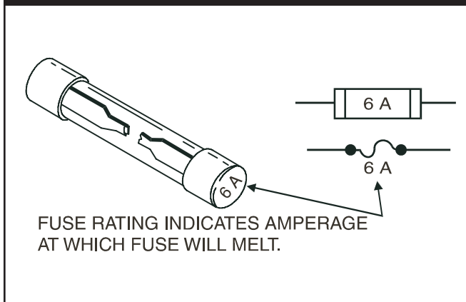
Figure 2.21 — A Typical Fuse
