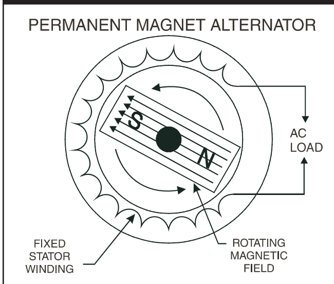
Figure 1.27 — Simple Revolving Field Alternator
