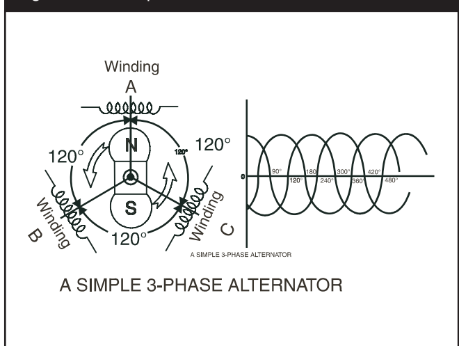
Figure 1.23 — Simple Three-Phase Alternator
