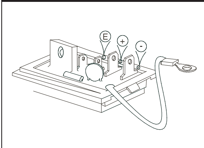
Figure 2.48 — Typical Bridge Rectifier
