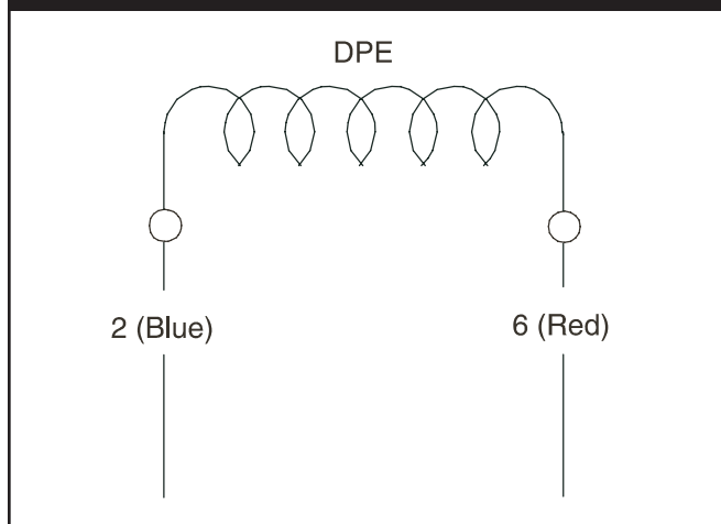
Figure 2.7 — Displaced Phase Excitation (DPE)
