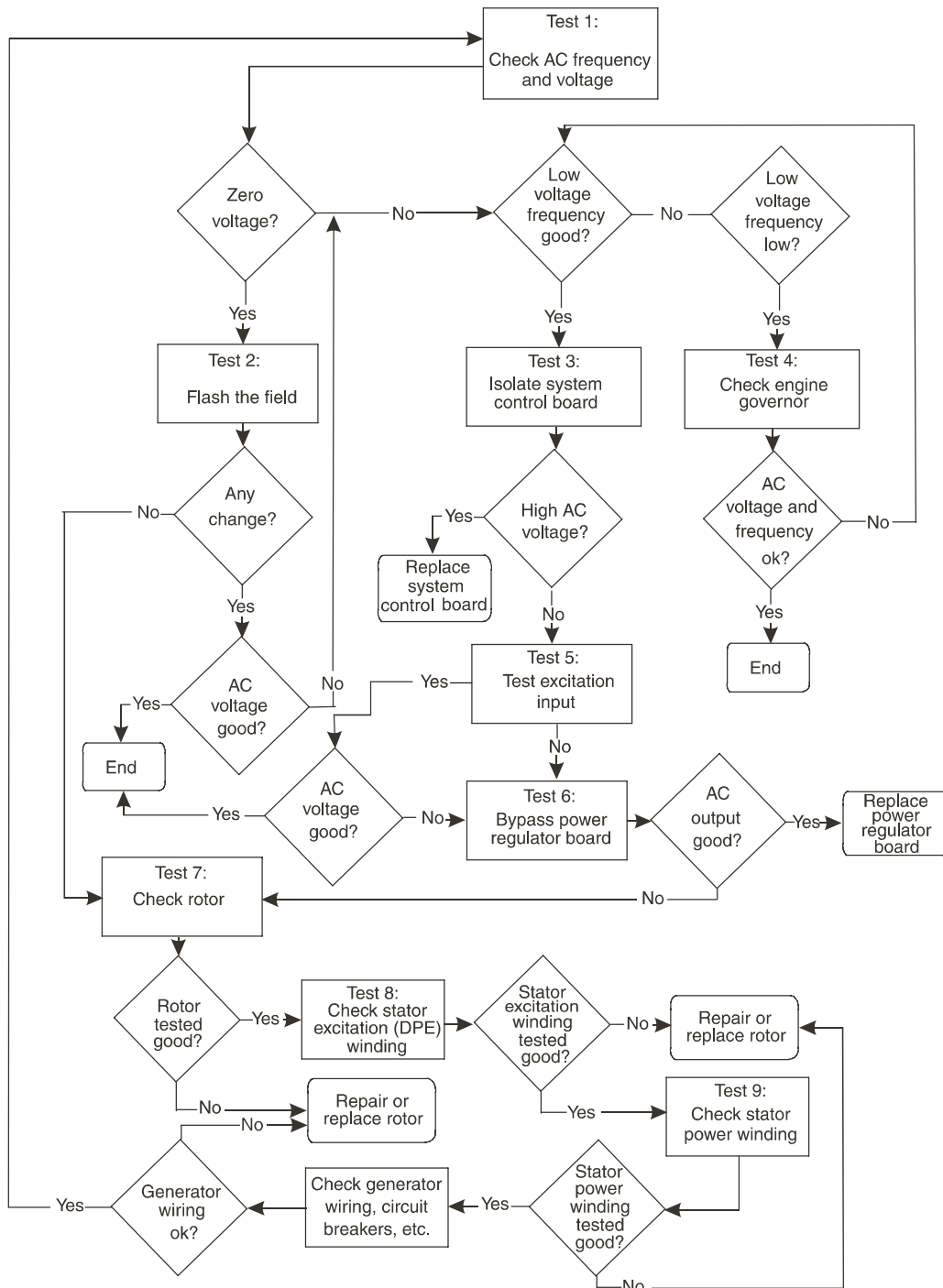
Figure 3.31—Troubleshooting Flow Chart For (Brush Type) Generators With “Two-Board” Regulation
