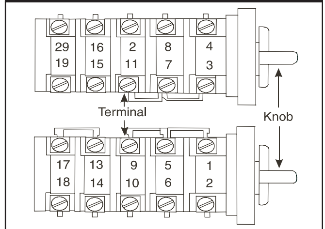
Figure 2.19 — Some Typical Rotary Switches
