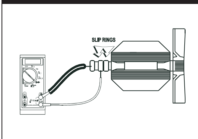
Figure 3.22 — Checking Rotor Short To Ground
