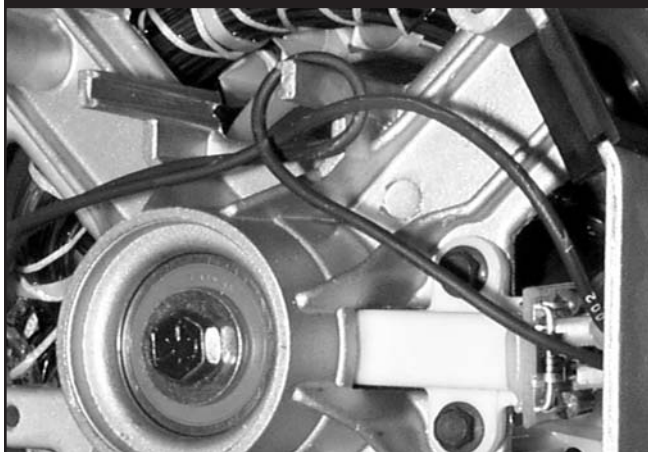
Figure 4.42 — Brush Holder Mounting
