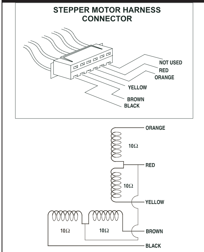
Figure 3.7 — Checking Stepper Motor
