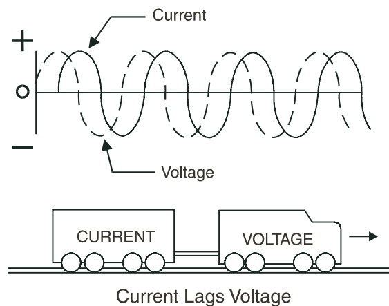
Figure 2.71 — Inductive Reactance
