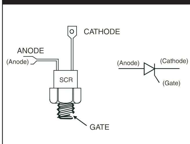
Figure 2.41 — Silicone-Controlled Rectifier
