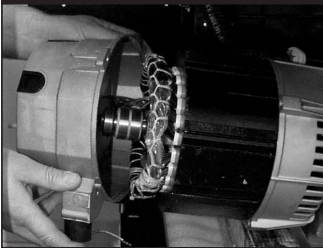
Figure 4.31 — Starting The Bearing Into Its Carrier
