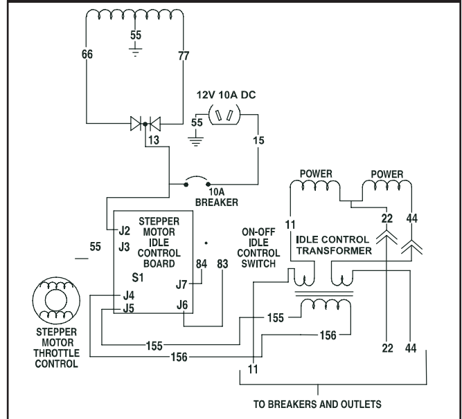
Figure 2.91 — Stepper Motor
