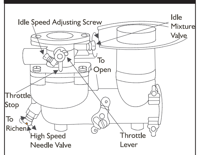
Figure 3.8 — Carburetor Adjustment
