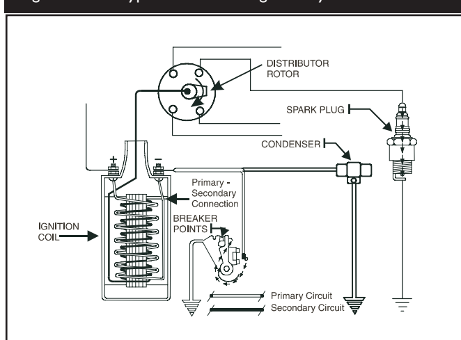
Figure 1.10 — Typical Automotive Ignition System
