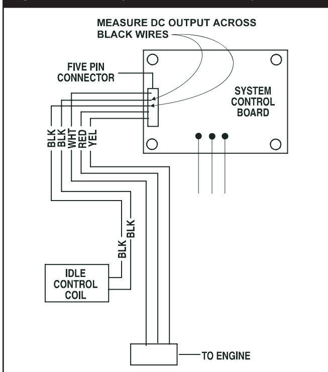
Figure 3.3 — Check System Control Board Output
