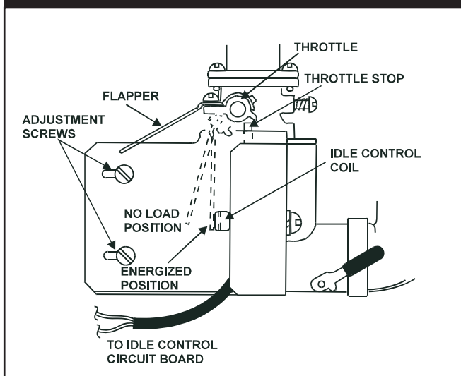
Figure 3.9 — Idle Control Coil And Flapper
