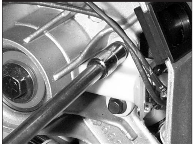
Figure 4.43 — Torque Brush Holder Assembly
