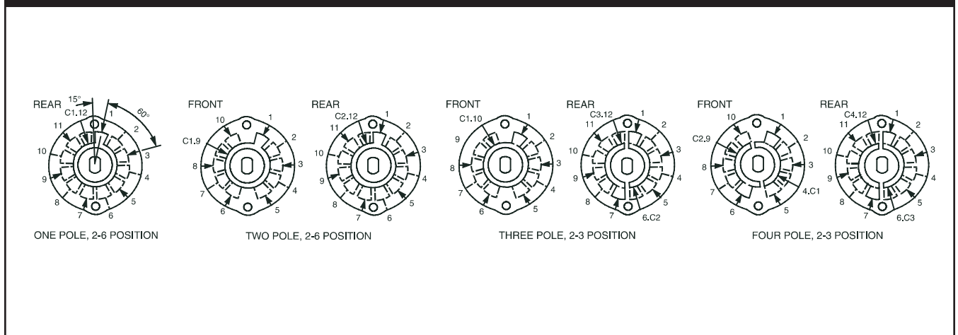
Figure 2.20 — Examples Of Rotary Switch Classifications
