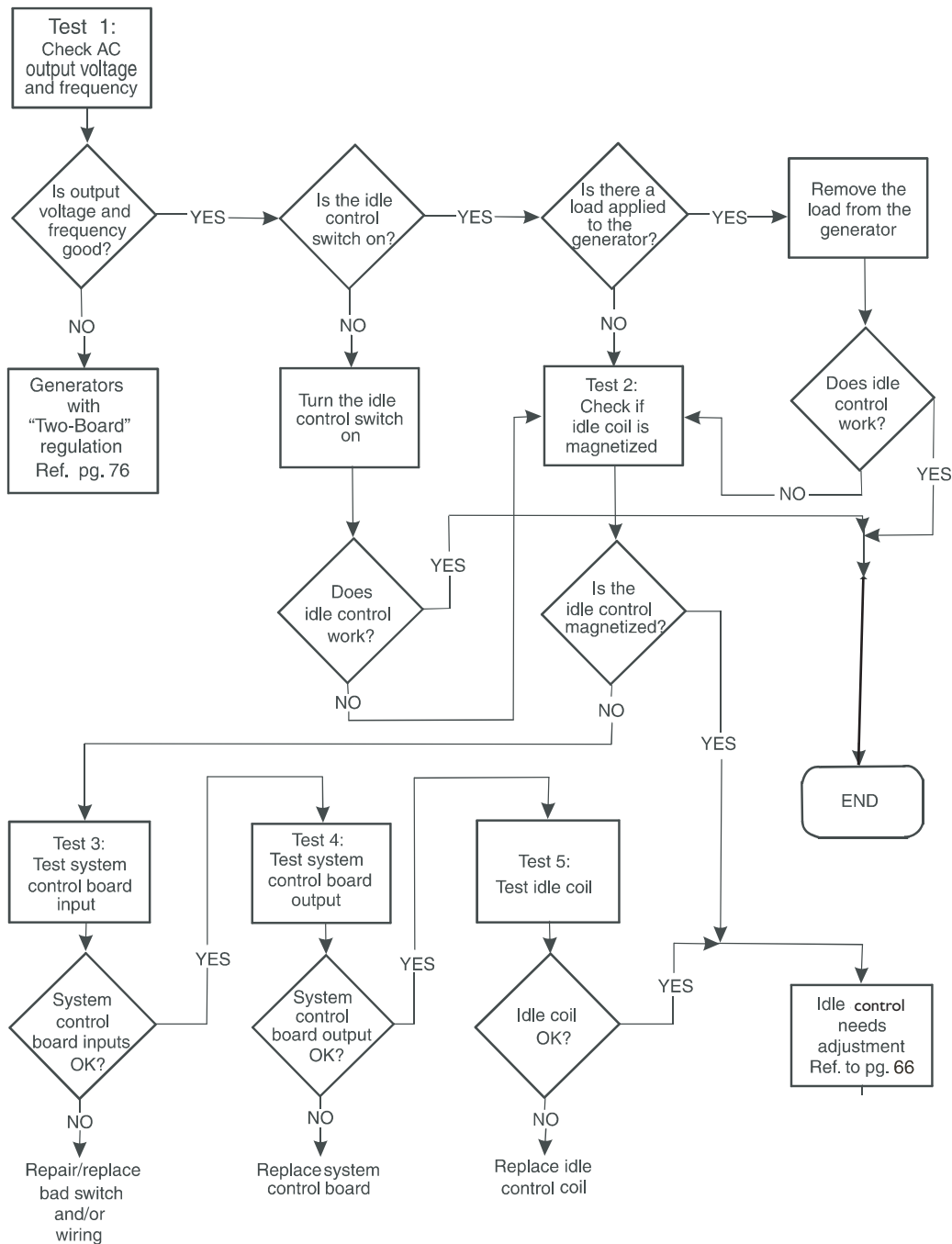
Figure 3.1 — Idle Control Troubleshooting Flow Chart (3500-7500 Watt Generators)
