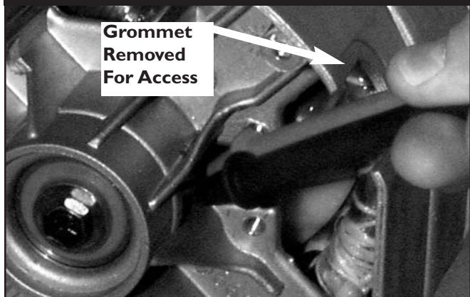
Figure 3.38 — Access To Rotor Slip Rings
