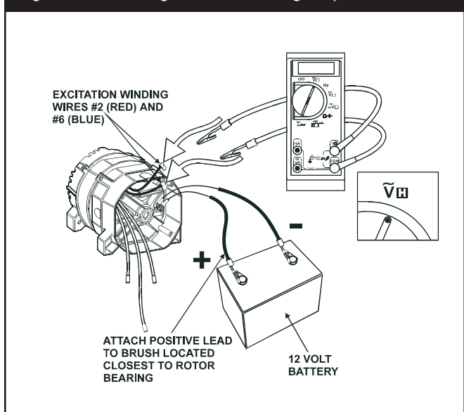
Figure 3.30 — Testing Excitation Winding Output
