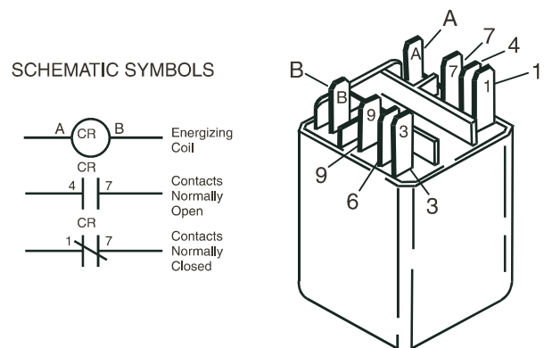
Figure 2.29 — Typical Relay With Schematic Symbols
