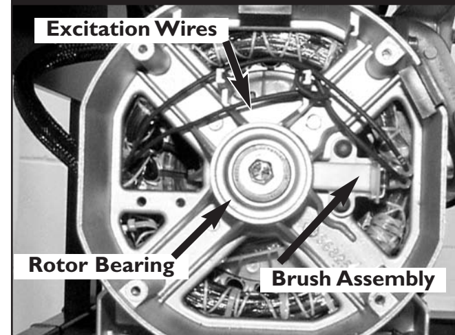
Figure 4.3 — Rear Bearing Carrier Exposed
