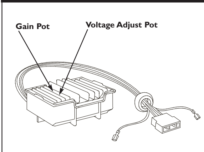
Figure 2.51 — Voltage Regulator
