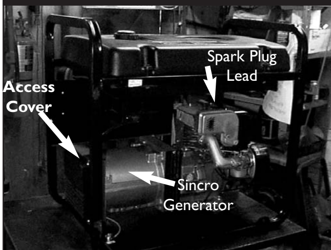
Figure 4.47 — Sincro® Wound Generator
