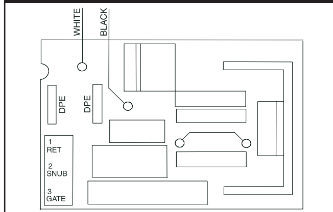
Figure 2.56 — Power Regulator Circuit Board
