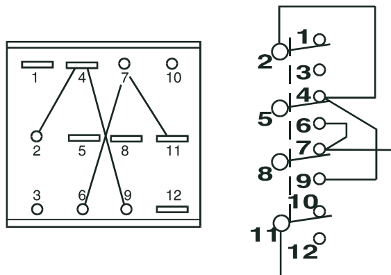
Figure 2.17 — Four Pole, Double Throw (4PDT)
