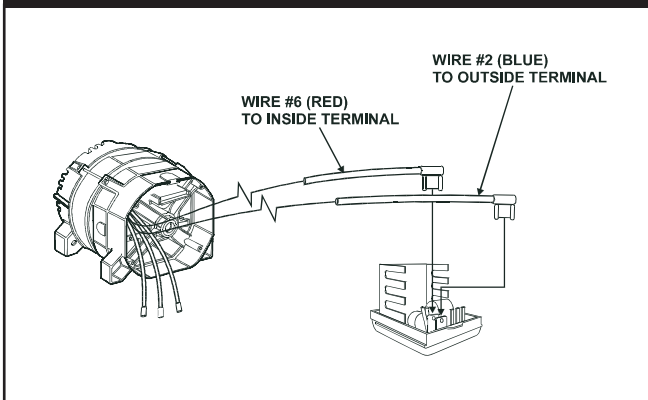
Figure 3.35 — Power Regulator Board Connections
