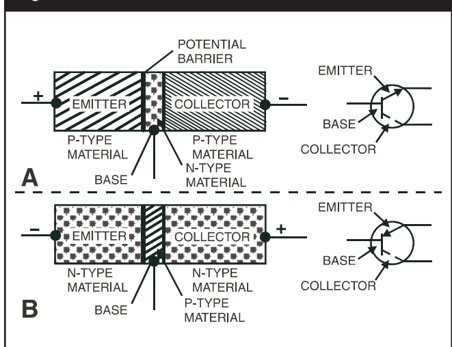
Figure 2.43 — Construction Of A Transistor
