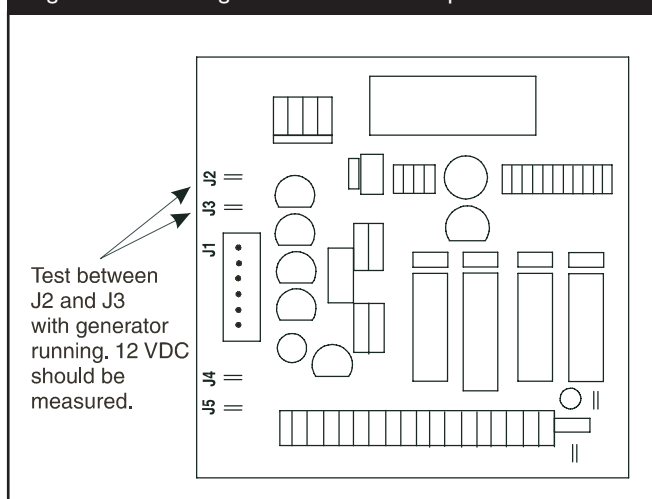
Figure 3.5 — Testing Idle Control Board Input
