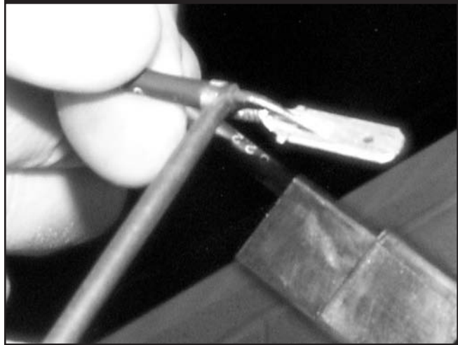
Figure 4.9 — Terminal Locking Tabs
