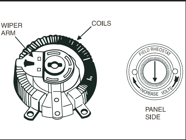
Figure 2.32 — Typical Rheostat
