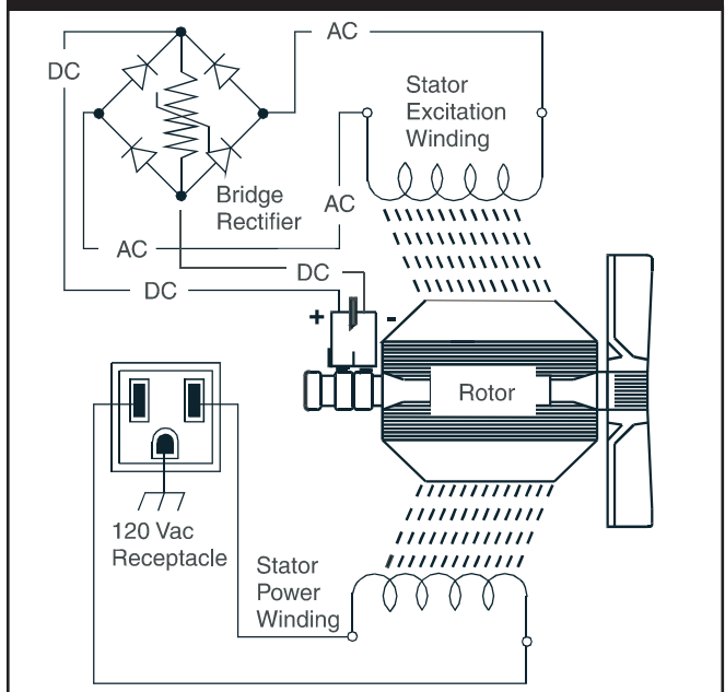
Figure 2.50 — Generator with a Bridge Rectifier
