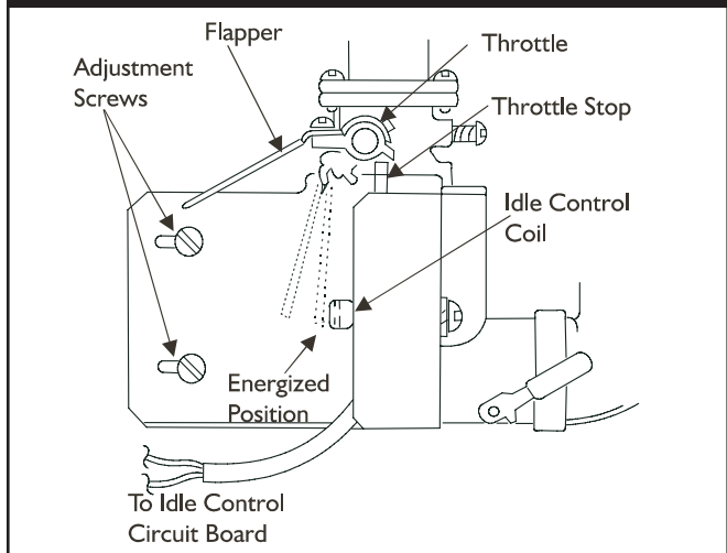
Figure 2.82 — Idle Control Coil And Flapper
