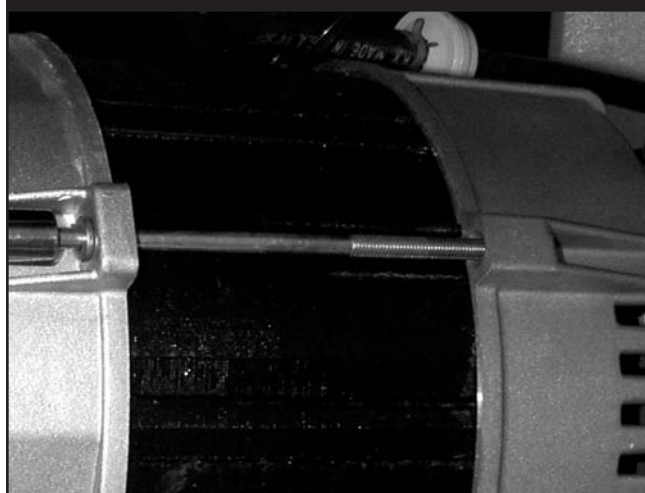
Figure 4.13 — Stator Bolts
