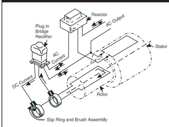
Figure 2.66 — Operation Of Reactor-Excited Alternator
