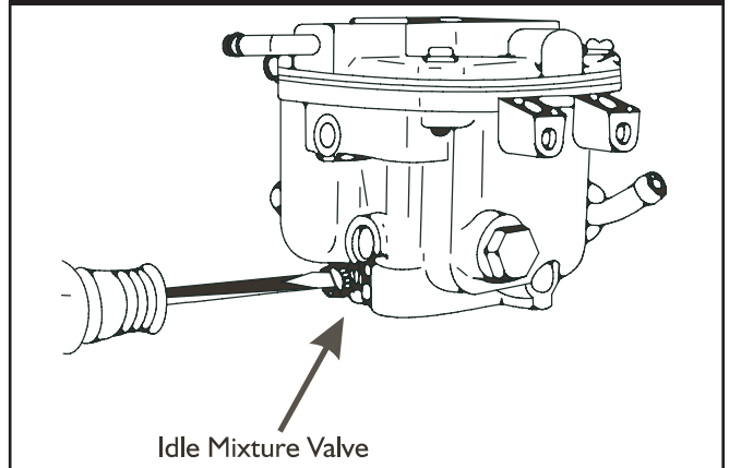
Figure 3.14 — Idle Mixture Adjustment
