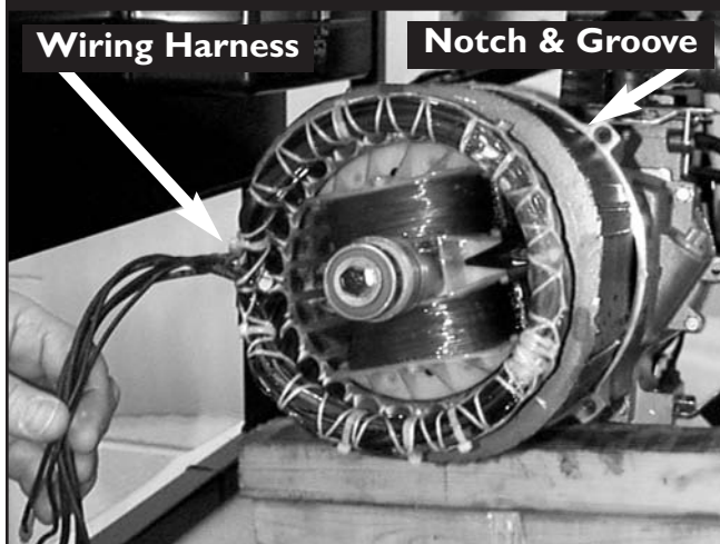
Figure 4.28 — Indexing The Stator
