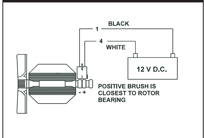
Figure 3.18 — Restoring Residual Magnetism
