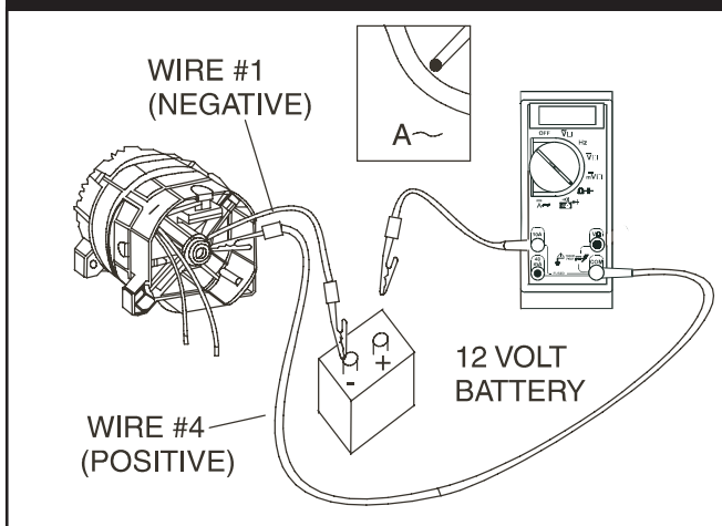
Figure 3.40 — Rotor Current Draw Test
