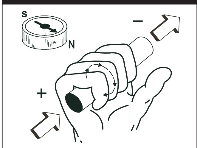
Figure I.7 — The Right Hand Rule
