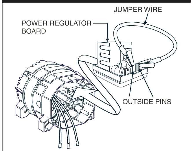
Figure 3.34 — Installing Jumper Wire
