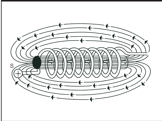
Figure I.12 — Iron Core Increases Strength of Field
