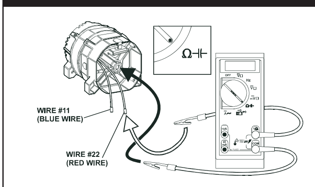
Figure 3.45 — Testing For Short To Ground
