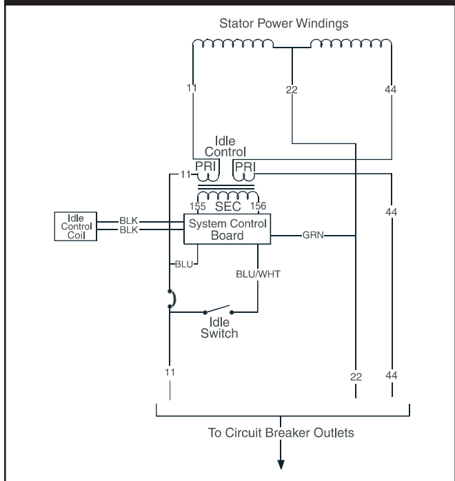
Figure 2.88 — Idle Control Schematic
