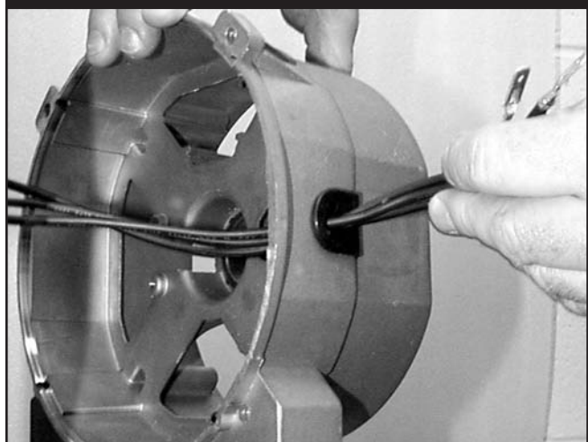
Figure 4.30 — Threading Harness Through Grommet
