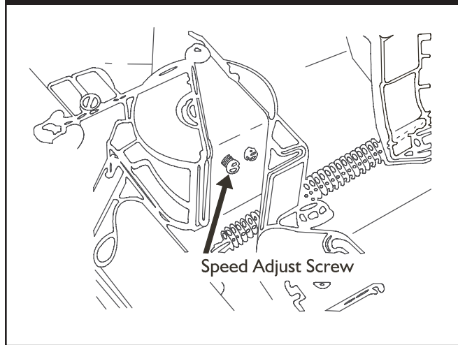
Figure 3.11 — No Load Frequency Adjustment Screw
