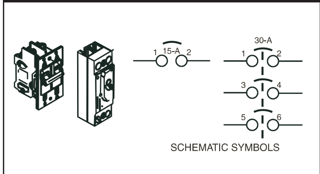
Figure 2.22 — Typical Circuit Breakers
