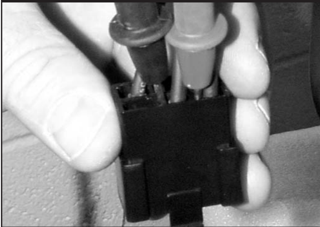
Figure 3.27 — Checking Power Winding Resistance
