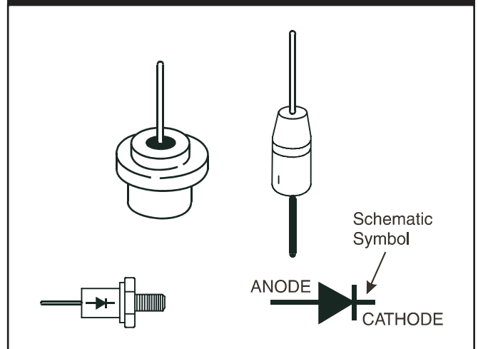
Figure 2.39 — Typical Blocking Diodes
