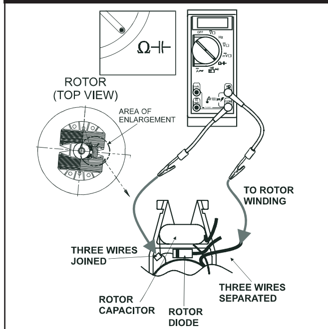
Figure 3.56 — Testing Rotor Windings
