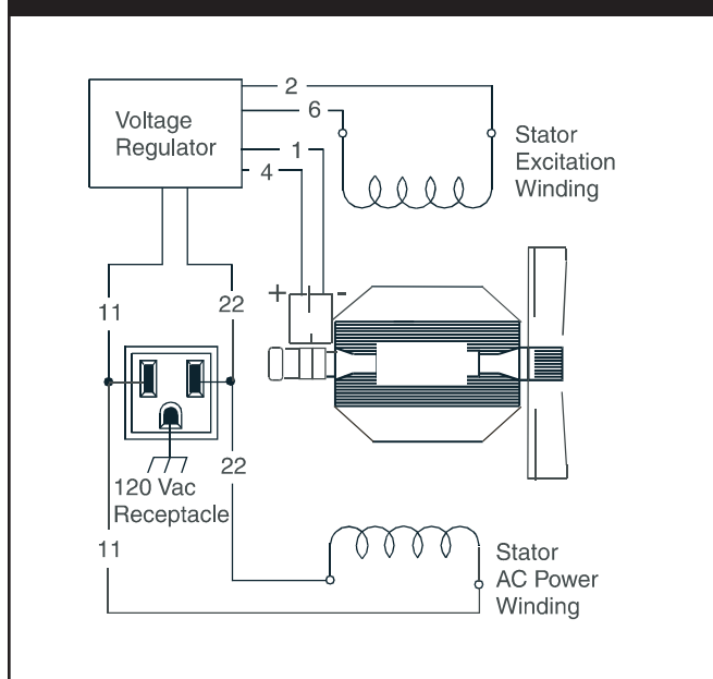
Figure 2.54 — Generator With Voltage Regulator
