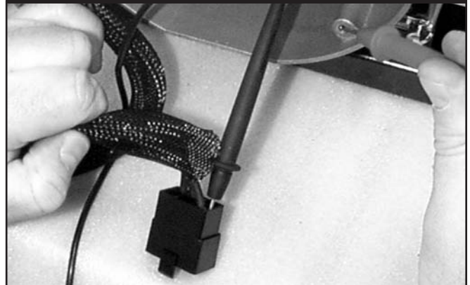
Figure 3.28 — Testing For Short To Ground
