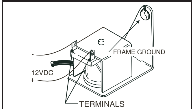
Figure 2.26 — Typical Fuel Shutoff Valve
