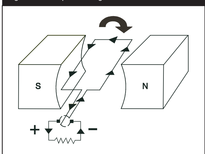
Figure I.8 — Simple Revolving Armature Generator
