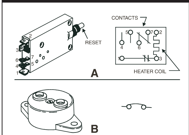
Figure 2.23 — Examples of Thermal Switches
