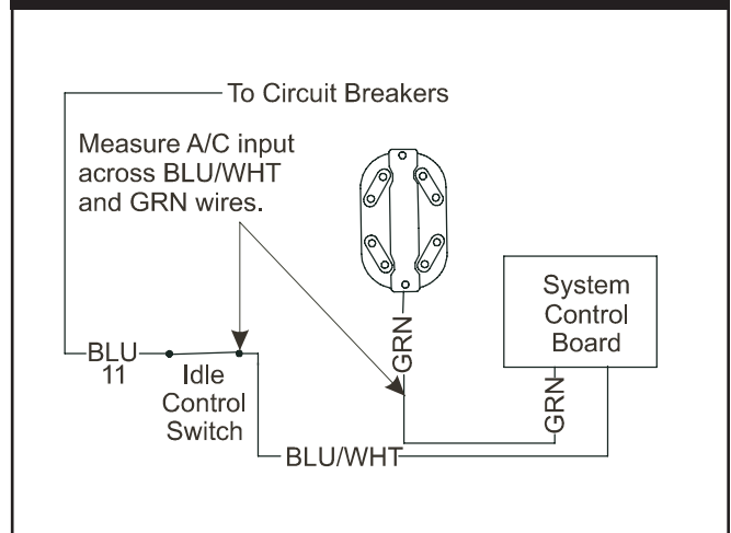
Figure 3.2 — Check System Control Board Input
