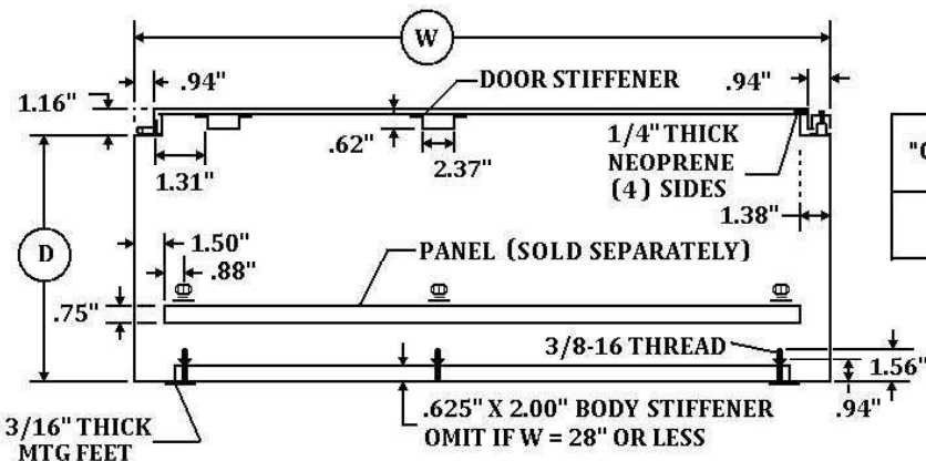
SECTION X-X
