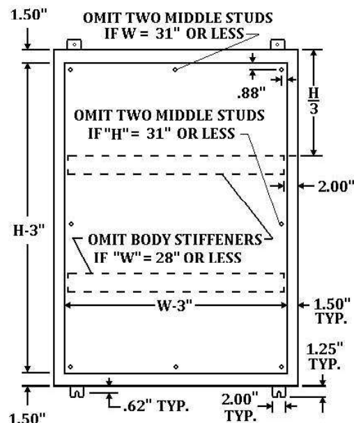
SECTION Y-Y
