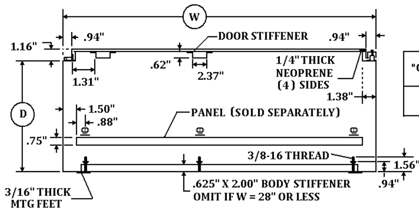
SECTION X-X
