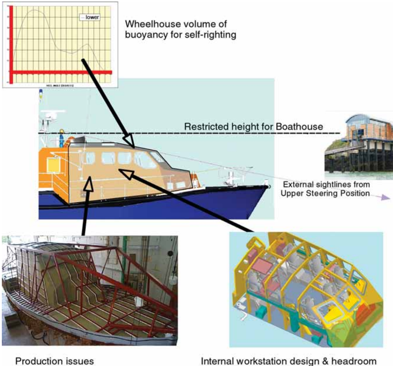
Figure K-2 RNLI design considerations for Tamar Class Lifeboat
