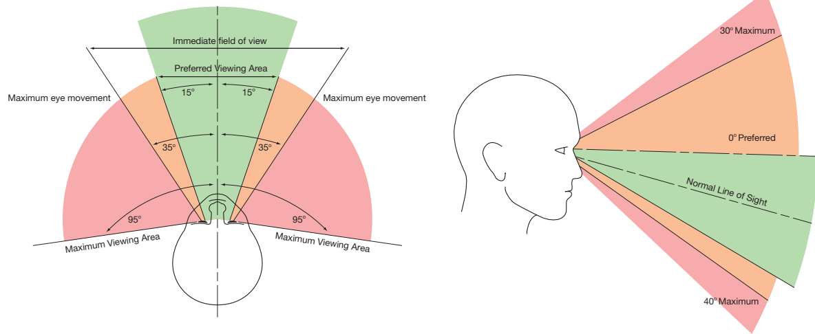
Figure F-6 Example of optimal horizontal and vertical field-of-view Ref: IMO MSC/Circ. 982 and MIL-STD-1472F
