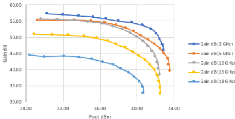
MB2.0018G434820 Gain dB over Power Out
