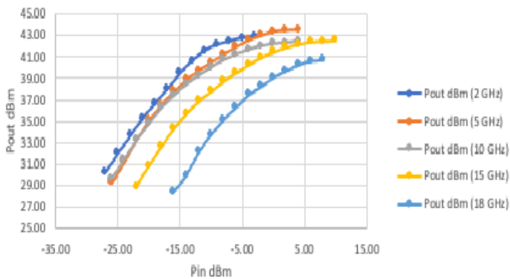
MB2.0018G434820 Psat dB over Frequency
