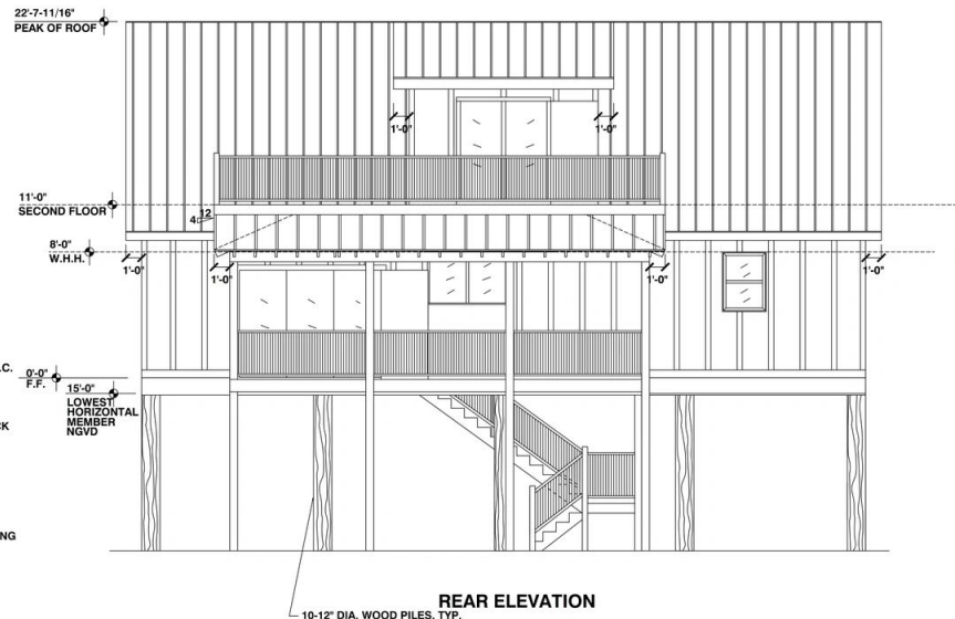
REAR ELEVATION
