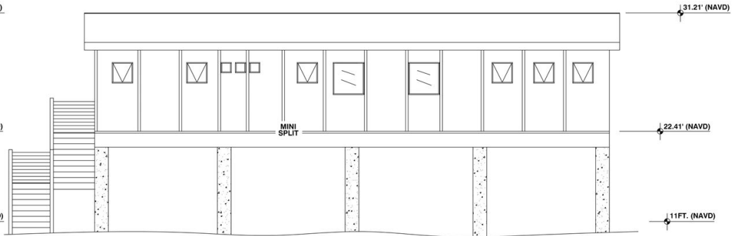
REAR ELEVATION
