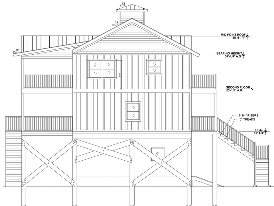
LEFT ELEVATION
