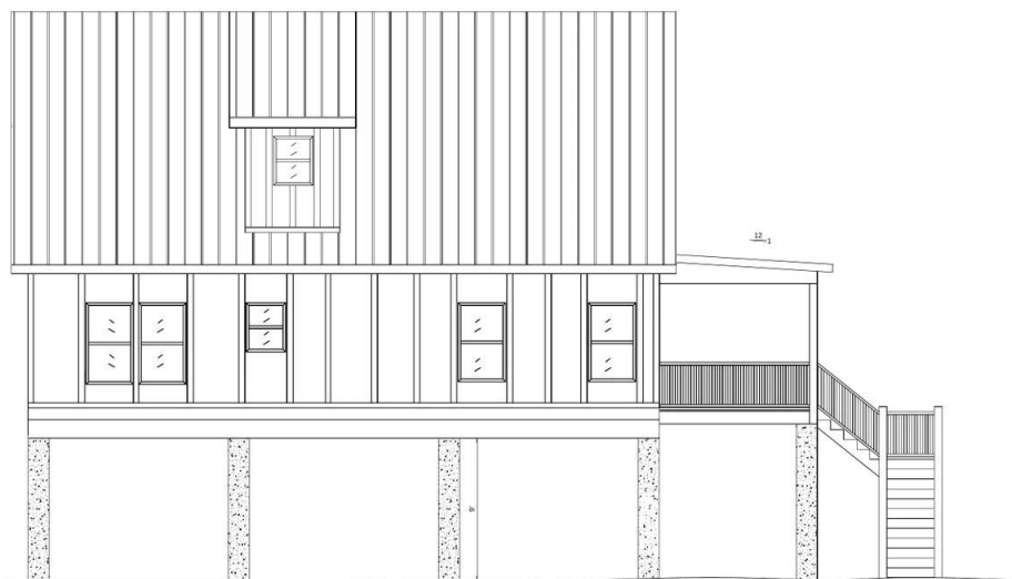
LEFT ELEVATION
