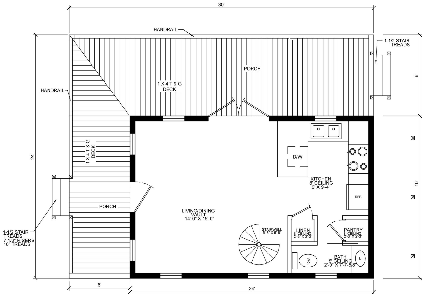
FIRST FLOOR 384 SQ. FT.
