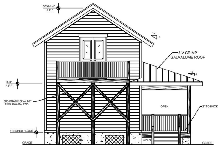
REAR (EAST) ELEVATION
