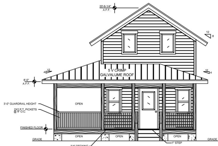
FRONT (WEST) ELEVATION
