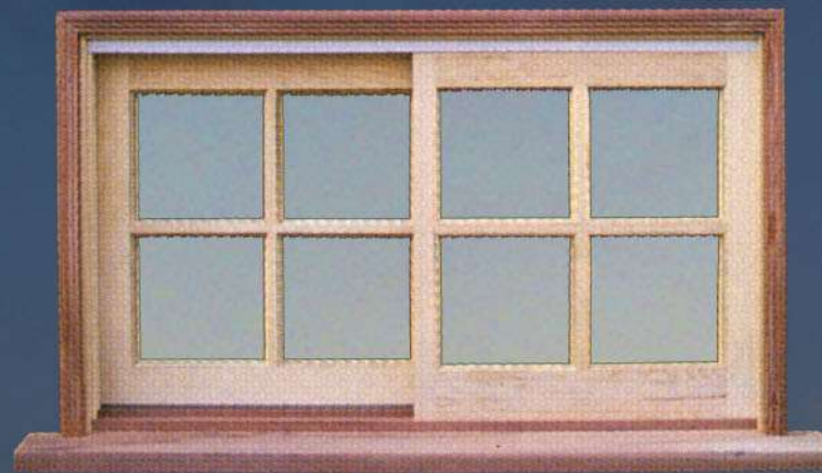
HORIZONTAL SLIDING WINDOWS With white vinyl tracks or with metal track and rollers Available handings: XO, OX, XOX, or OXXO
