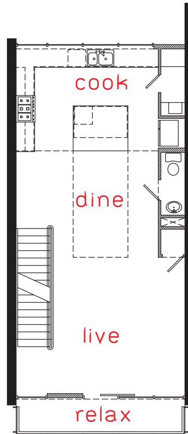
second 774 ft 2 conditioned 76 ft 2 balcony
