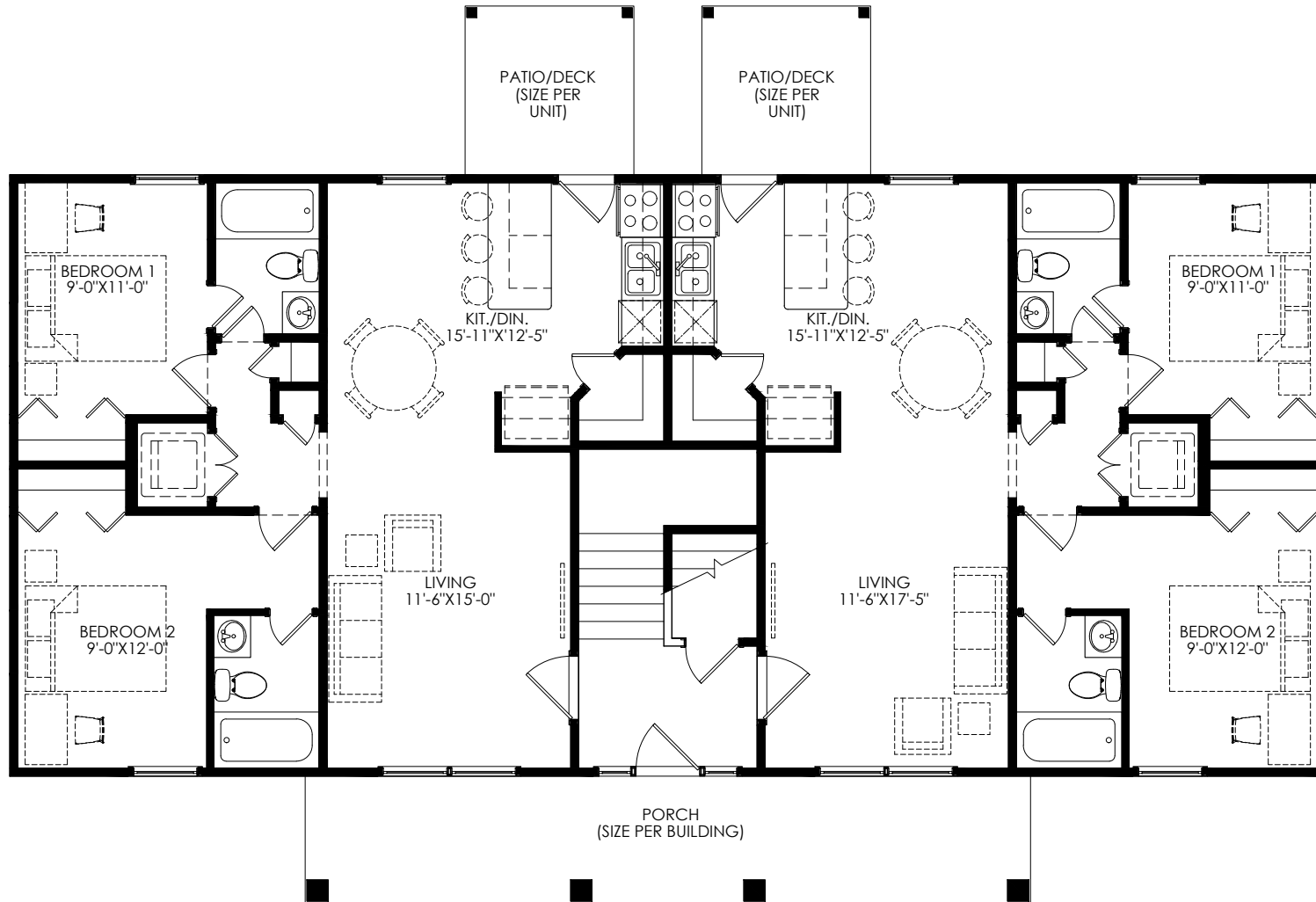
TYPICAL BUILDING PLAN
