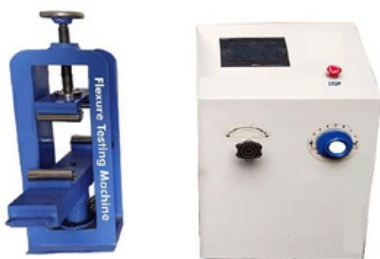
Flexure Testing Machine (Digitally Operated) FI-207
