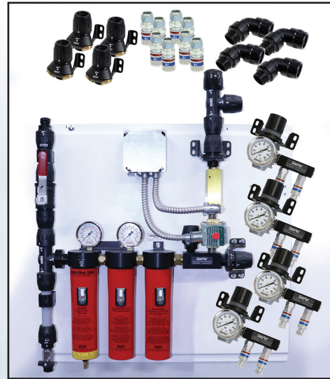
SATA/DanAmAir Filtration Panel for Two Booths Part #801620
