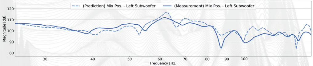
Narrowband Frequency Response
