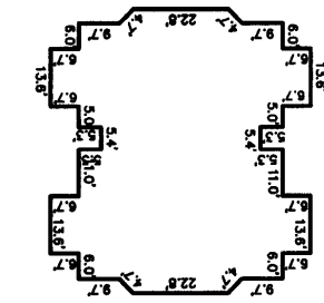
BUILDING TYPE V BUILDINGS # 14, 19, 20.
