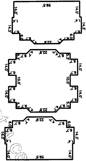
BUILDING TYPE IV BUILDINGS # 4, 6, 7, 8, 11, 15, 18, 21.
