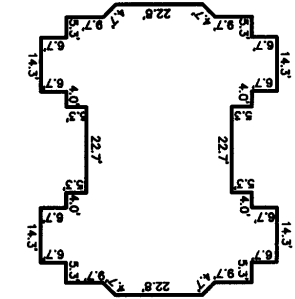
BUILDING TYPE II BUILDINGS # 2, 5, 13, 16.
