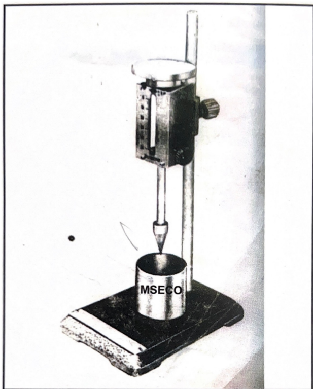
SOIL PENTROMETER
