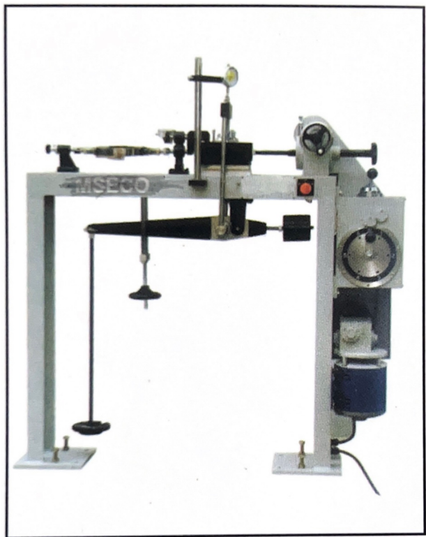
DIRECT SHEAR (MOTORISED)
