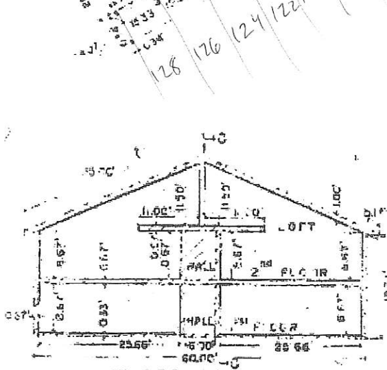
CROSS SECTION SCALE 1/8" = 1'-0" C-B
