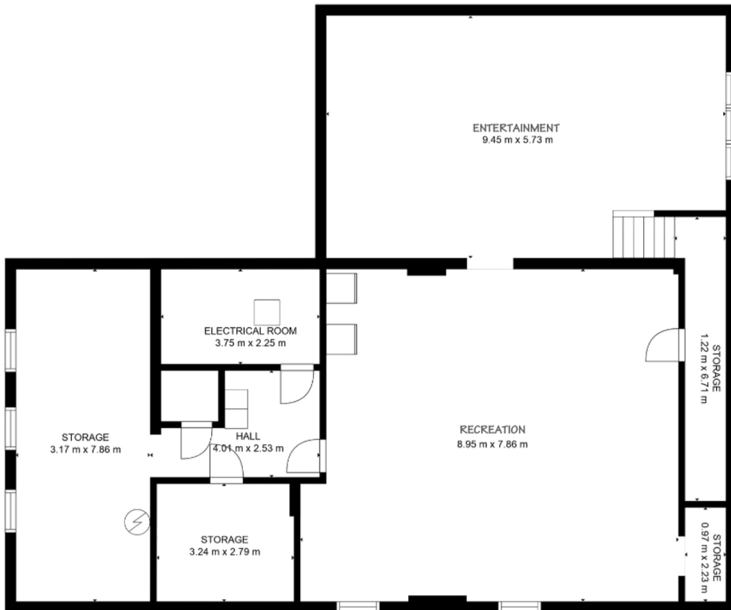
BASEMENT
