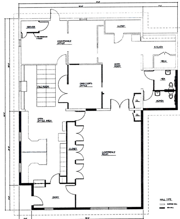
Proposed Floor Plan with New Addition Not to Scale
