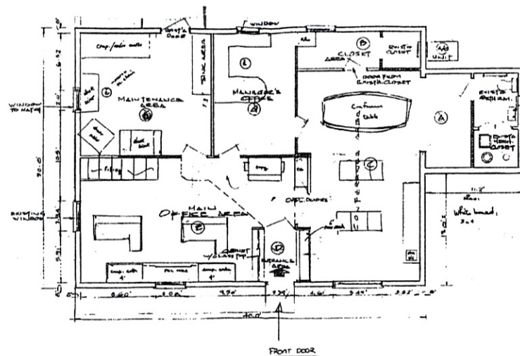
Existing Floor Plan Not to Scale
