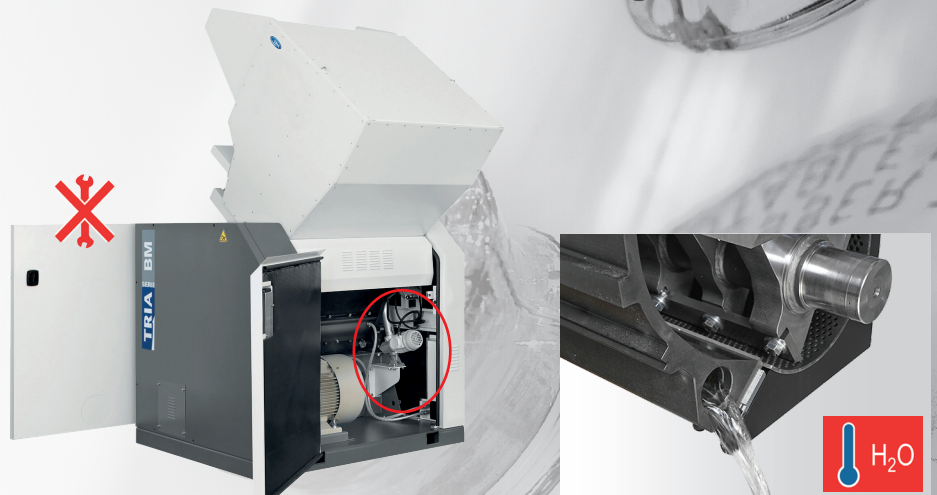
Hopper opening by motorized jack; integrated security system, with two fuse opening/closing. Access without tools to the main parts subject to ordinary maintenance.
