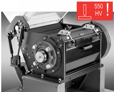
Grinding chamber in 550HV antiwear execution; hopper opening by gas cylinder.
