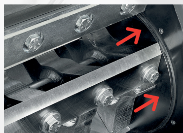
Rotary discs integral with the rotor and containment rings; bench adjustment of blades and counterblades. Scissor cutting configuration.
