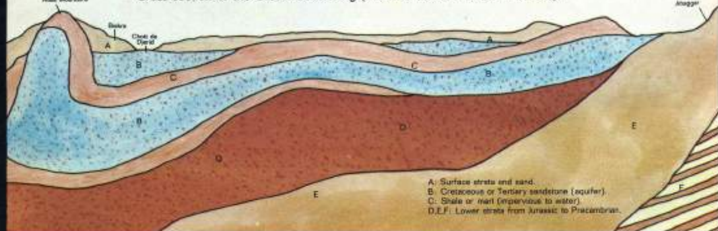
Cross section of the Great Eastern Erg (see blue line on northern Sahara).
