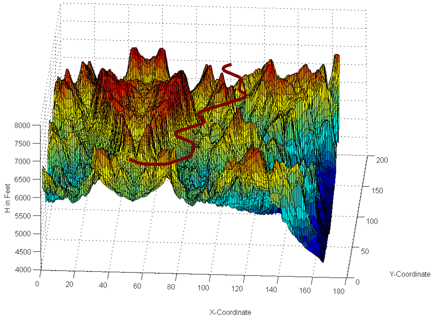
Path Planner Algorithm - FP at 7000 Feet
