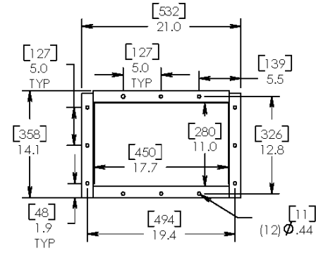
DISCHARGE FLANGE BOLT PATTERN
