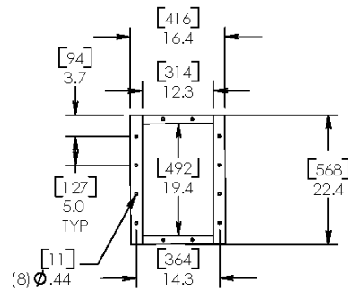
INLET OPENING SECTION B-B
