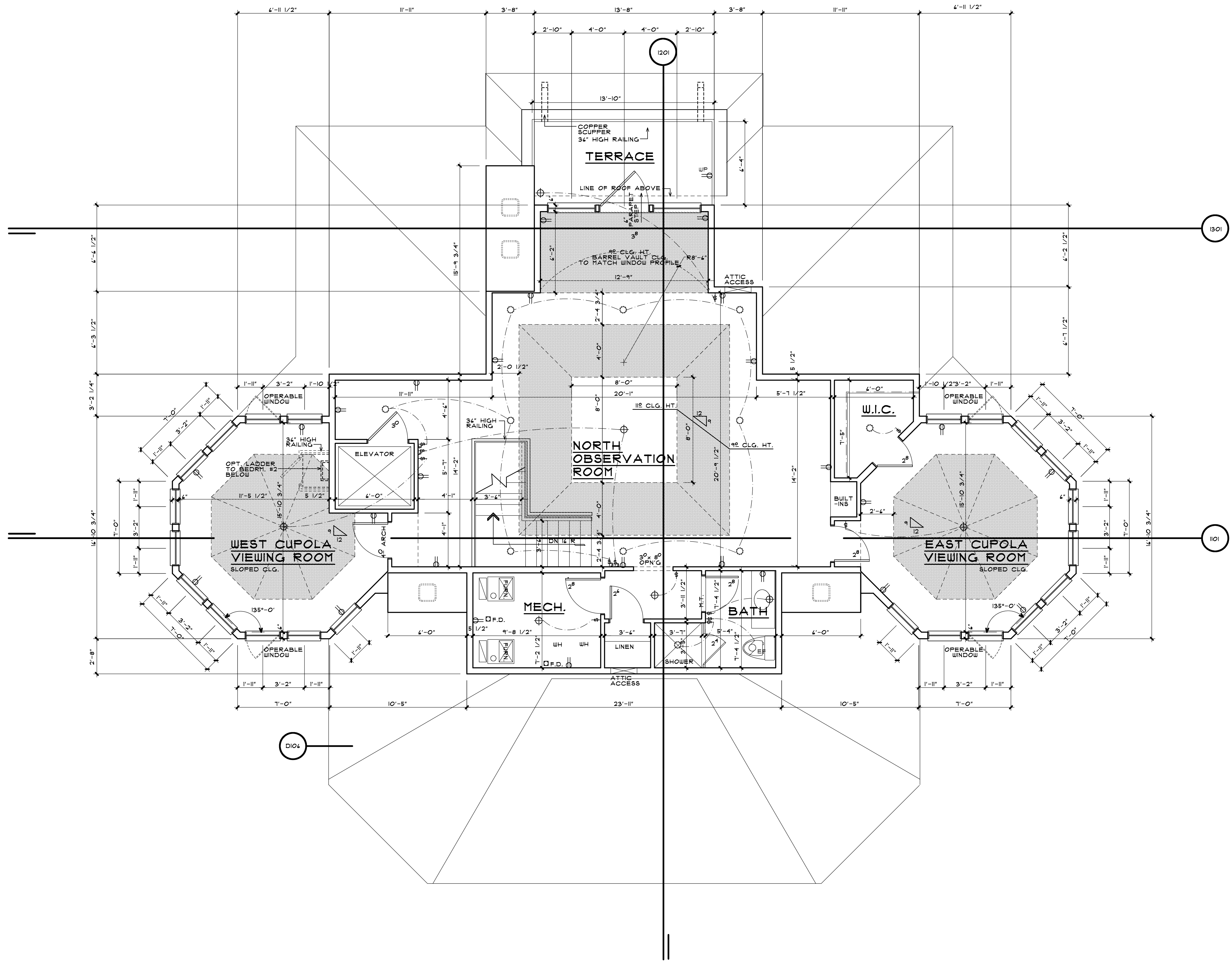
THIRD FLOOR PLAN
