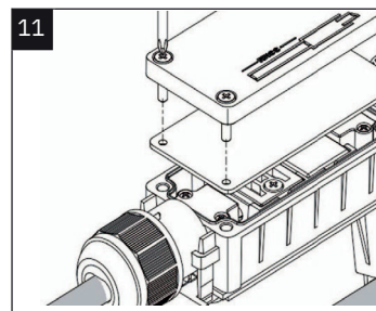
11. After the installation of cables at both side, cover the connector cover plate and tighten the four screws alternately to ensure that the sealing ring is compressed.
