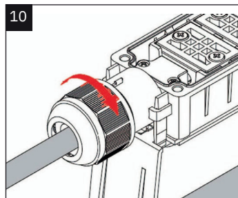
10. Repeat steps 2-10 to install the cable at the other side.
