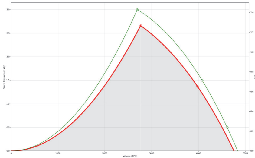
100% Fan Curve Overlap
