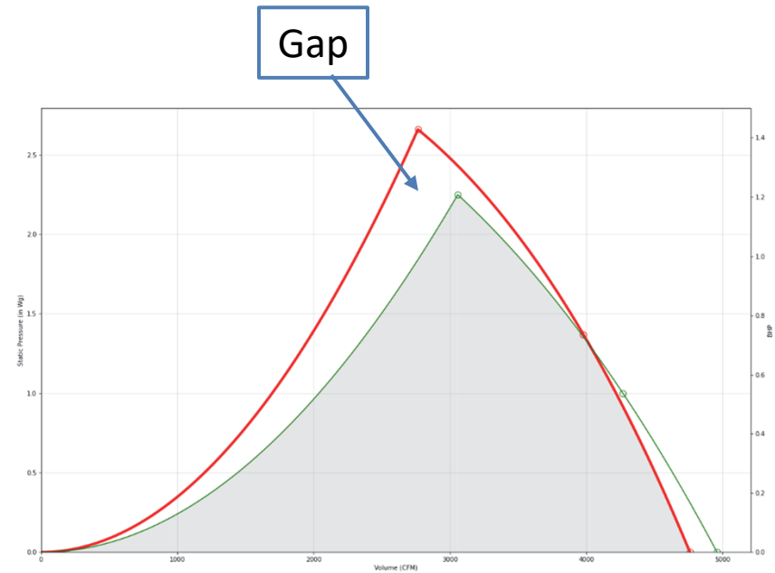
82% Fan Curve Overlap
