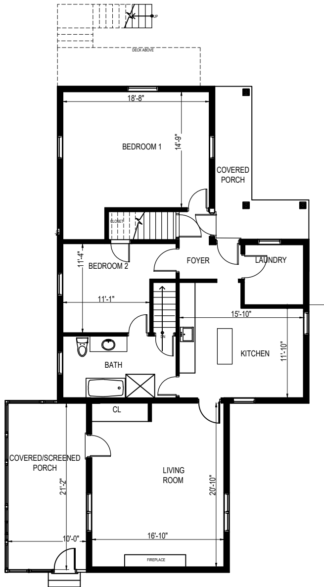
UNIT D - GROUND FLOOR PLAN 1450 sq.ft.
