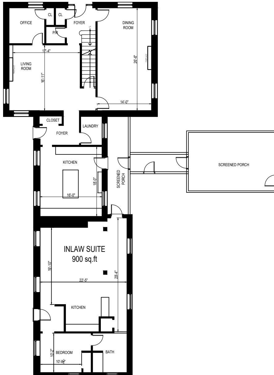
GROUND FLOOR PLAN 2700 sq.ft.
