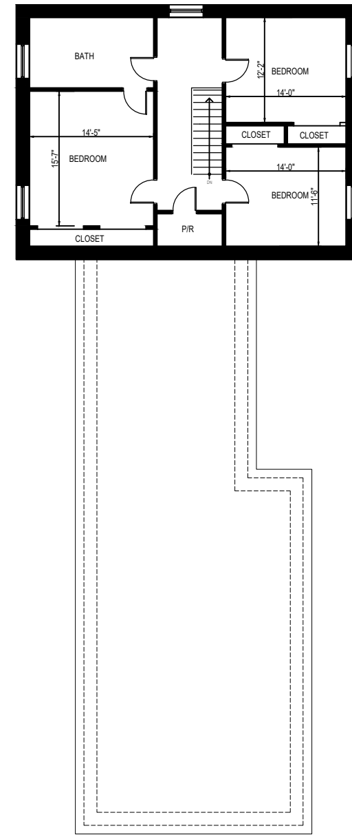
SECOND FLOOR PLAN 1170 sq. ft.
