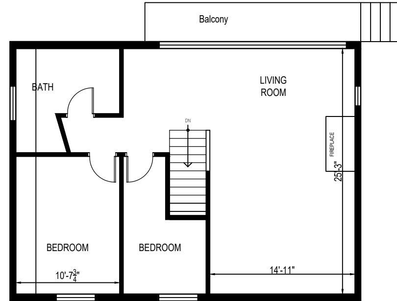
SECOND FLOOR PLAN 960 sq. ft.
